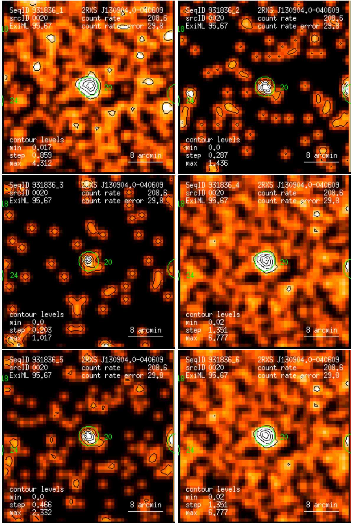
Figure 20: RASS 931836: detection 0020: band rate images, Gaussian filter: (1) PSPC channels 11 – 41, (2) 52 – 90, (3) 91 – 201, (4) 11 – 235, (5) 52 – 201, (6) 11 – 201. Broad band rates in counts/ks. Band rate contour levels in counts/ks/arcmin 2 .
