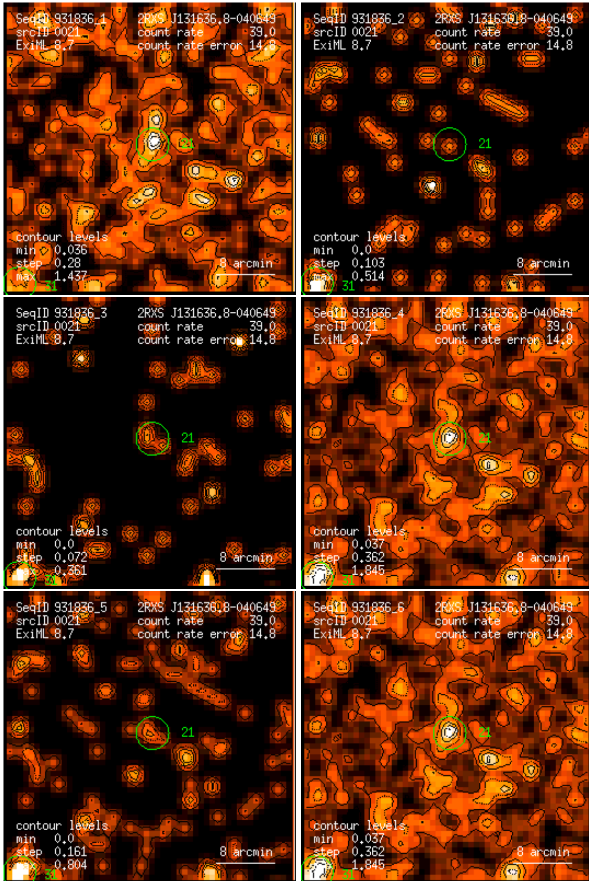
Figure 21: RASS 931836: detection 0021: band rate images, Gaussian filter: (1) PSPC channels 11 – 41, (2) 52 – 90, (3) 91 – 201, (4) 11 – 235, (5) 52 – 201, (6) 11 – 201. Broad band rates in counts/ks. Band rate contour levels in counts/ks/arcmin 2 .
