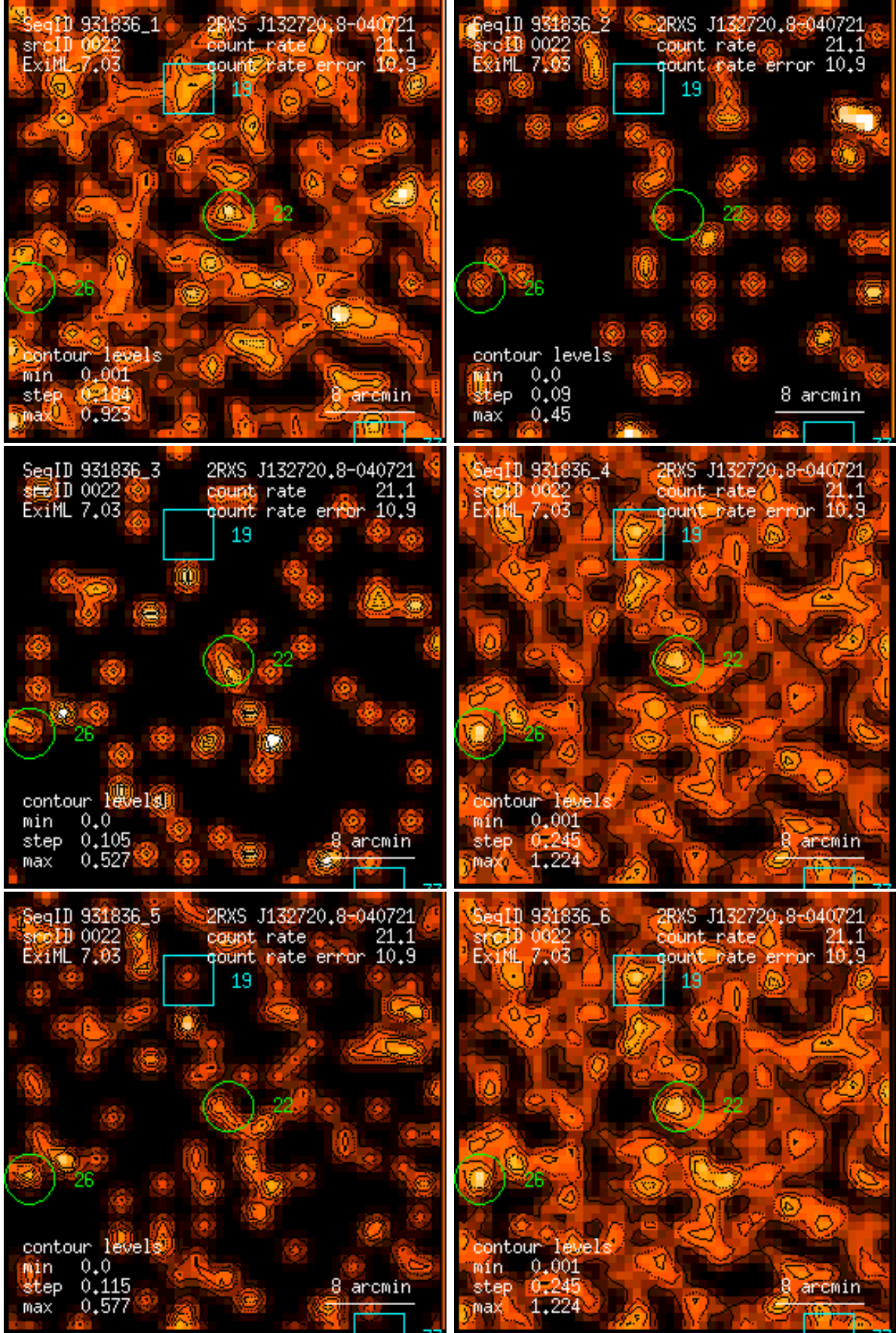
Figure 22: RASS 931836: detection 0022: band rate images, Gaussian filter: (1) PSPC channels 11 – 41, (2) 52 – 90, (3) 91 – 201, (4) 11 – 235, (5) 52 – 201, (6) 11 – 201. Broad band rates in counts/ks. Band rate contour levels in counts/ks/arcmin 2 .
