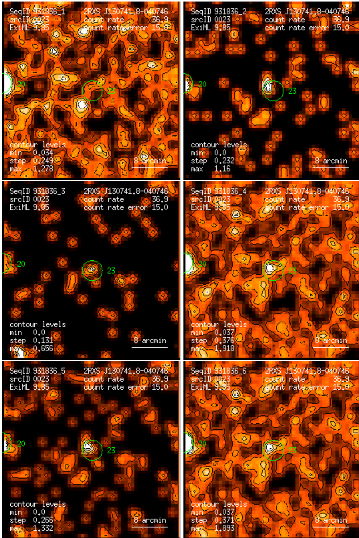
Figure 23: RASS 931836: detection 0023: band rate images, Gaussian filter: (1) PSPC channels 11 – 41, (2) 52 – 90, (3) 91 – 201, (4) 11 – 235, (5) 52 – 201, (6) 11 – 201. Broad band rates in counts/ks. Band rate contour levels in counts/ks/arcmin 2 .
