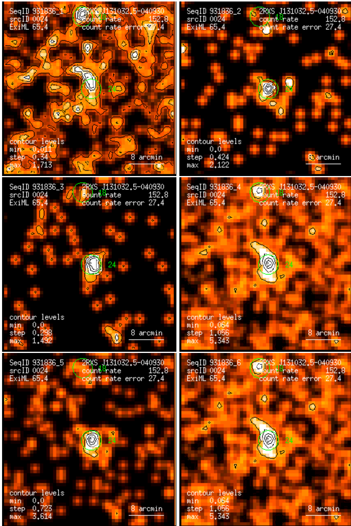
Figure 24: RASS 931836: detection 0024: band rate images, Gaussian filter: (1) PSPC channels 11 – 41, (2) 52 – 90, (3) 91 – 201, (4) 11 – 235, (5) 52 – 201, (6) 11 – 201. Broad band rates in counts/ks. Band rate contour levels in counts/ks/arcmin 2 .
