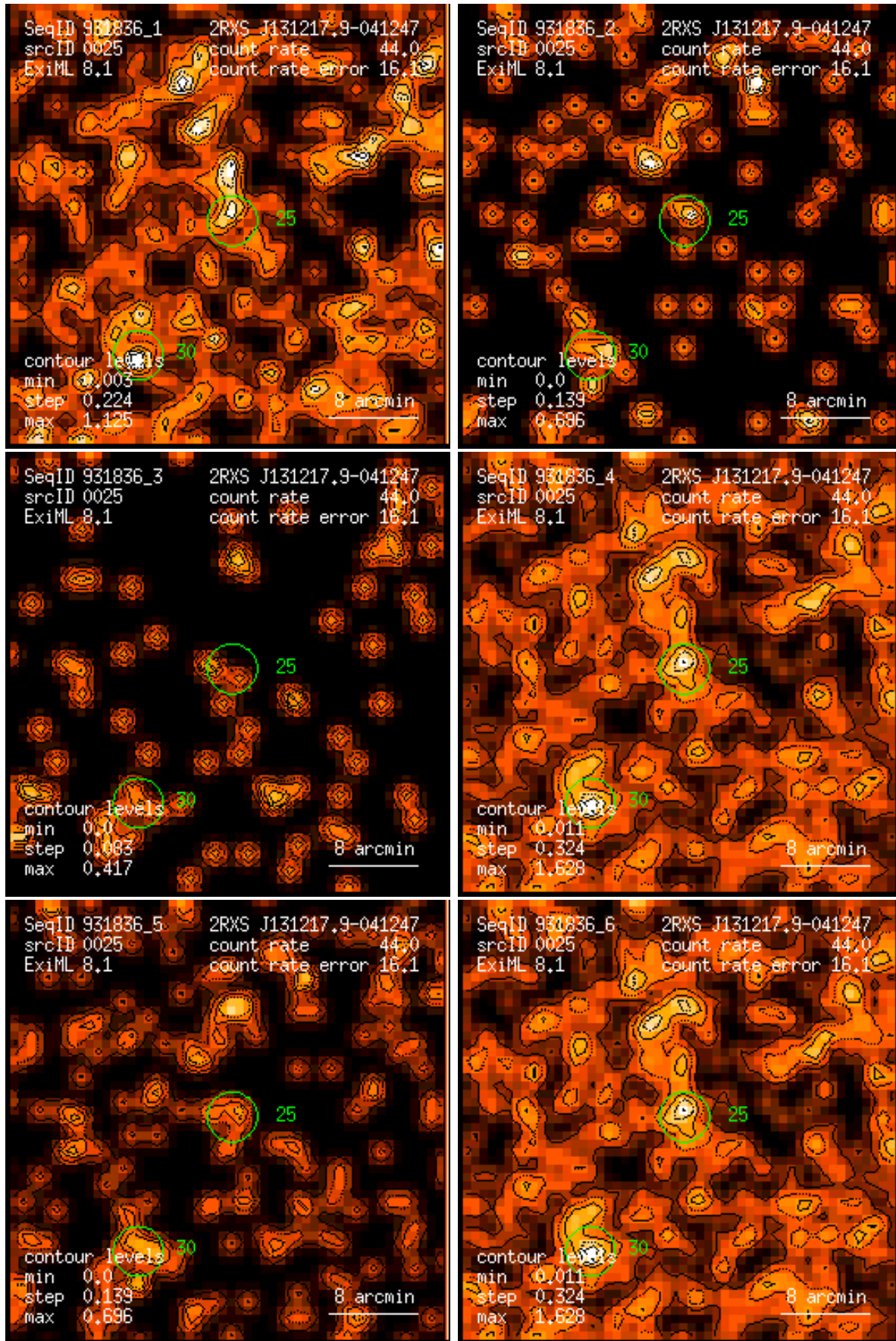
Figure 25: RASS 931836: detection 0025: band rate images, Gaussian filter: (1) PSPC channels 11 – 41, (2) 52 – 90, (3) 91 – 201, (4) 11 – 235, (5) 52 – 201, (6) 11 – 201. Broad band rates in counts/ks. Band rate contour levels in counts/ks/arcmin 2 .
