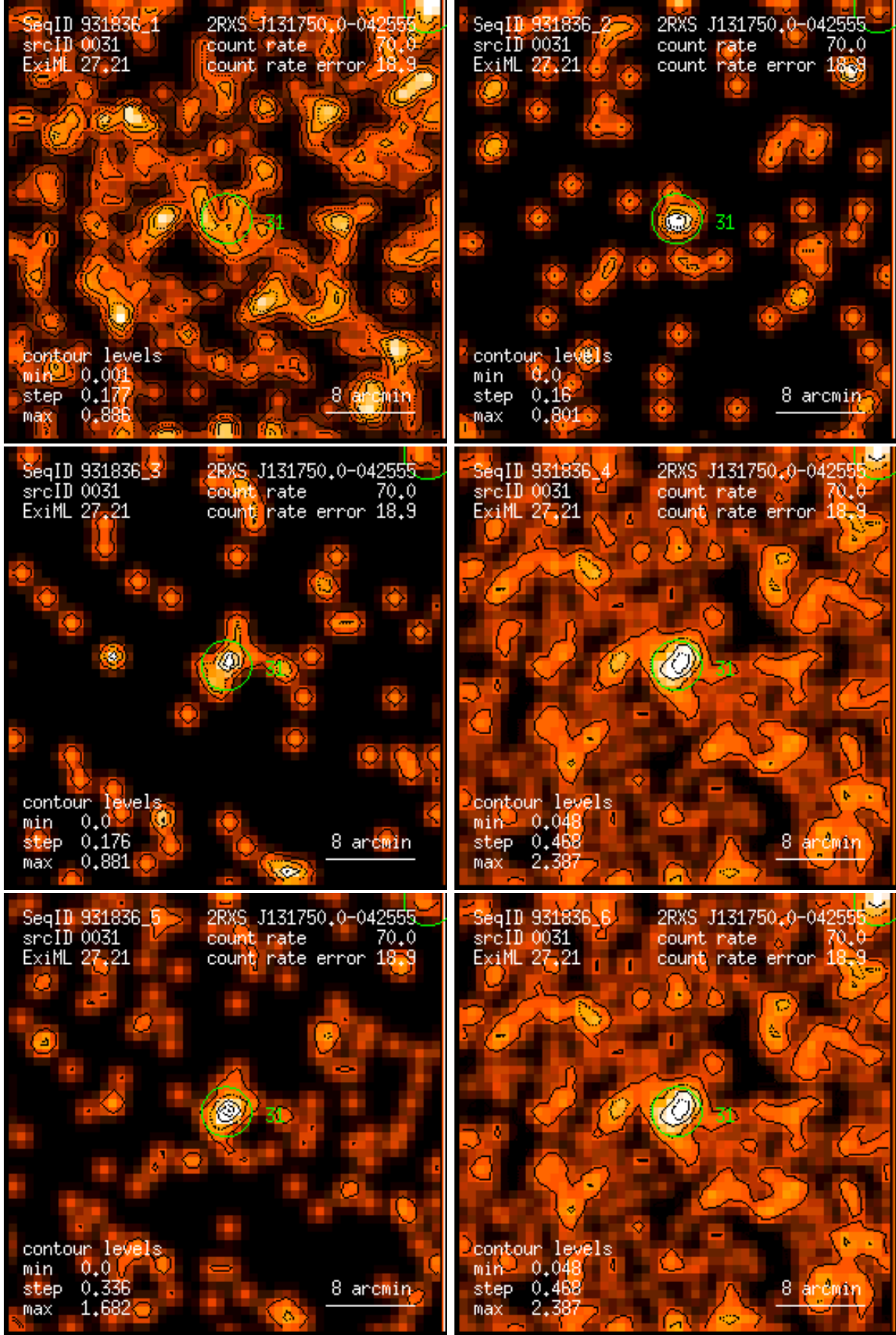
Figure 31: RASS 931836: detection 0031: band rate images, Gaussian filter: (1) PSPC channels 11 – 41, (2) 52 – 90, (3) 91 – 201, (4) 11 – 235, (5) 52 – 201, (6) 11 – 201. Broad band rates in counts/ks. Band rate contour levels in counts/ks/arcmin 2 .
