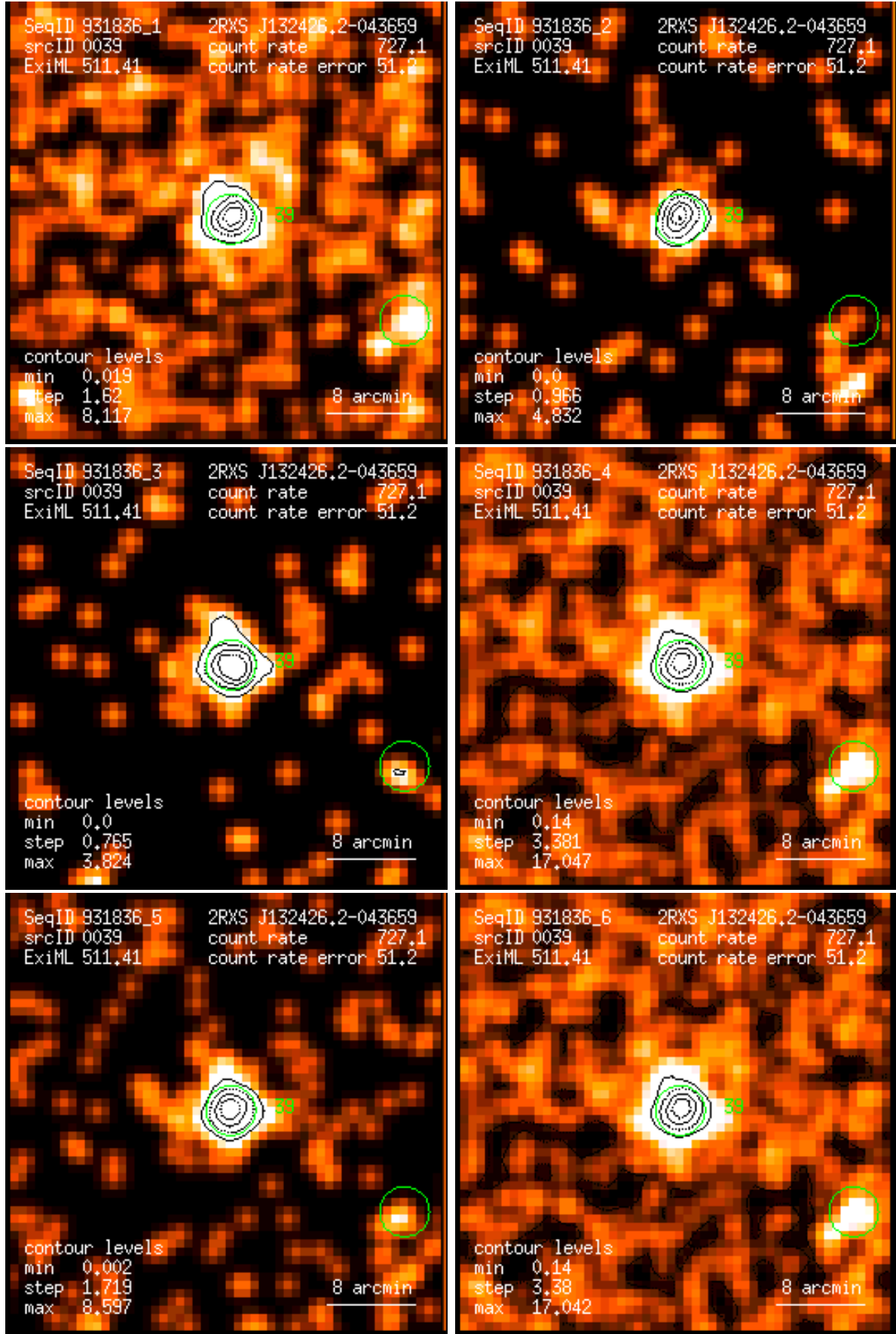
Figure 39: RASS 931836: detection 0039: band rate images, Gaussian filter: (1) PSPC channels 11 – 41, (2) 52 – 90, (3) 91 – 201, (4) 11 – 235, (5) 52 – 201, (6) 11 – 201. Broad band rates in counts/ks. Band rate contour levels in counts/ks/arcmin 2 .
