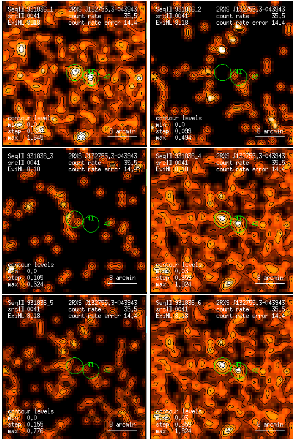
Figure 41: RASS 931836: detection 0041: band rate images, Gaussian filter: (1) PSPC channels 11 – 41, (2) 52 – 90, (3) 91 – 201, (4) 11 – 235, (5) 52 – 201, (6) 11 – 201. Broad band rates in counts/ks. Band rate contour levels in counts/ks/arcmin 2 .
