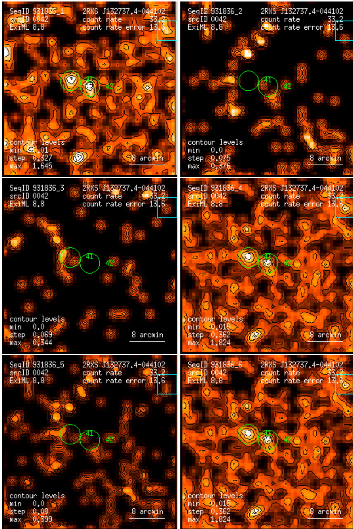
Figure 42: RASS 931836: detection 0042: band rate images, Gaussian filter: (1) PSPC channels 11 – 41, (2) 52 – 90, (3) 91 – 201, (4) 11 – 235, (5) 52 – 201, (6) 11 – 201. Broad band rates in counts/ks. Band rate contour levels in counts/ks/arcmin 2 .
