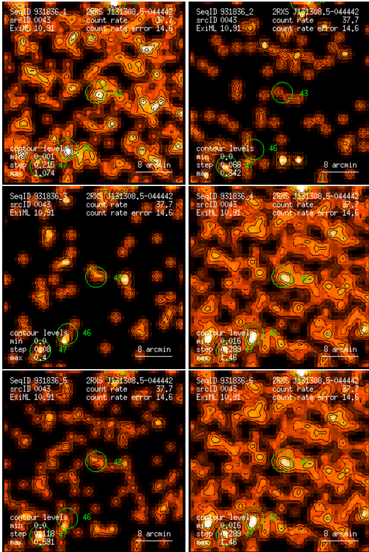
Figure 43: RASS 931836: detection 0043: band rate images, Gaussian filter: (1) PSPC channels 11 – 41, (2) 52 – 90, (3) 91 – 201, (4) 11 – 235, (5) 52 – 201, (6) 11 – 201. Broad band rates in counts/ks. Band rate contour levels in counts/ks/arcmin 2 .
