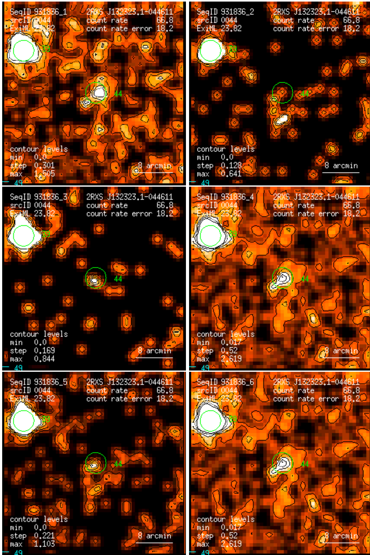
Figure 44: RASS 931836: detection 0044: band rate images, Gaussian filter: (1) PSPC channels 11 – 41, (2) 52 – 90, (3) 91 – 201, (4) 11 – 235, (5) 52 – 201, (6) 11 – 201. Broad band rates in counts/ks. Band rate contour levels in counts/ks/arcmin 2 .
