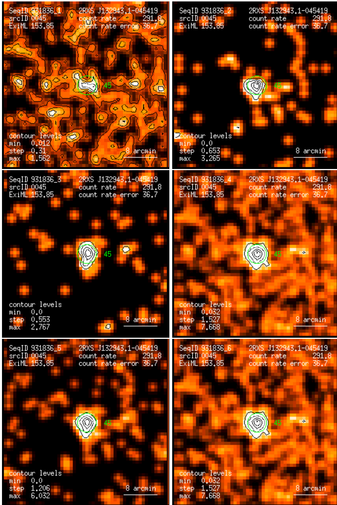
Figure 45: RASS 931836: detection 0045: band rate images, Gaussian filter: (1) PSPC channels 11 – 41, (2) 52 – 90, (3) 91 – 201, (4) 11 – 235, (5) 52 – 201, (6) 11 – 201. Broad band rates in counts/ks. Band rate contour levels in counts/ks/arcmin 2 .
