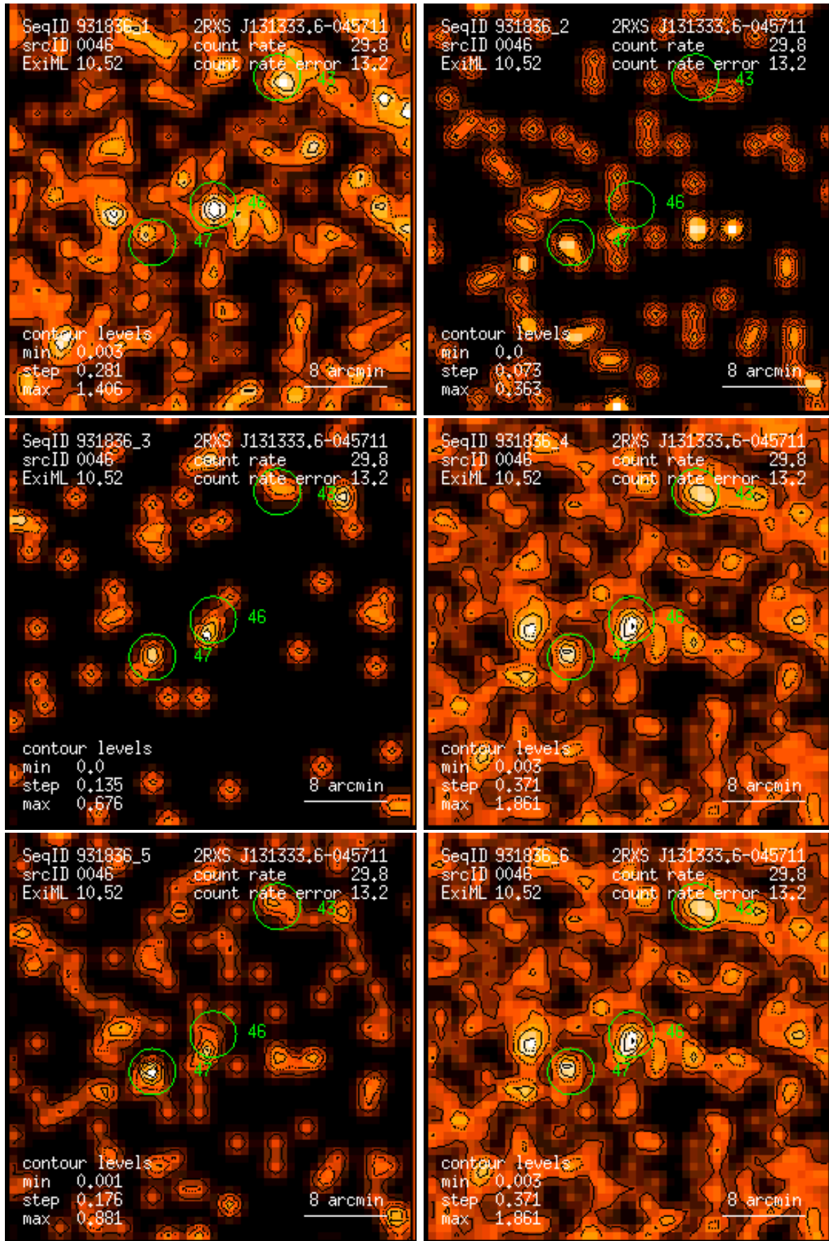
Figure 46: RASS 931836: detection 0046: band rate images, Gaussian filter: (1) PSPC channels 11 – 41, (2) 52 – 90, (3) 91 – 201, (4) 11 – 235, (5) 52 – 201, (6) 11 – 201. Broad band rates in counts/ks. Band rate contour levels in counts/ks/arcmin 2 .
