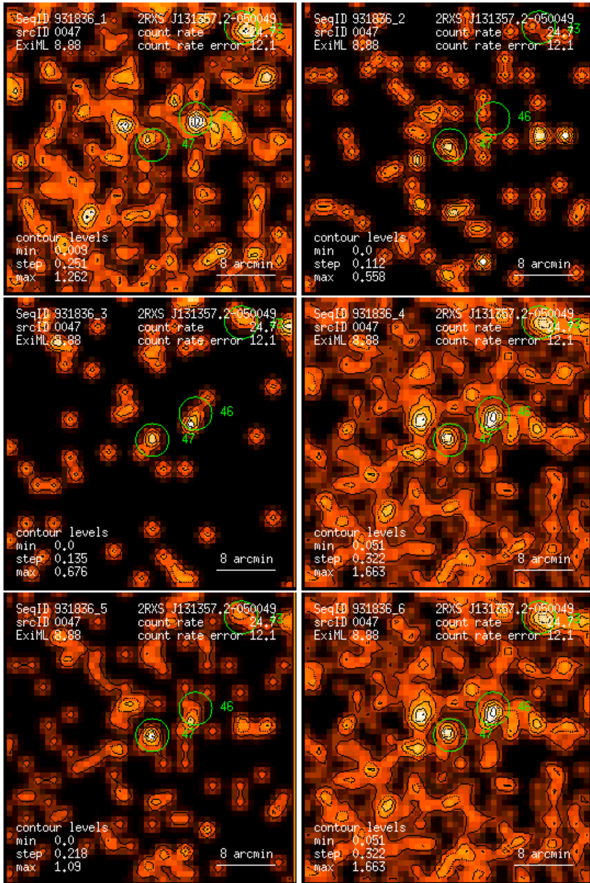
Figure 47: RASS 931836: detection 0047: band rate images, Gaussian filter: (1) PSPC channels 11 – 41, (2) 52 – 90, (3) 91 – 201, (4) 11 – 235, (5) 52 – 201, (6) 11 – 201. Broad band rates in counts/ks. Band rate contour levels in counts/ks/arcmin 2 .
