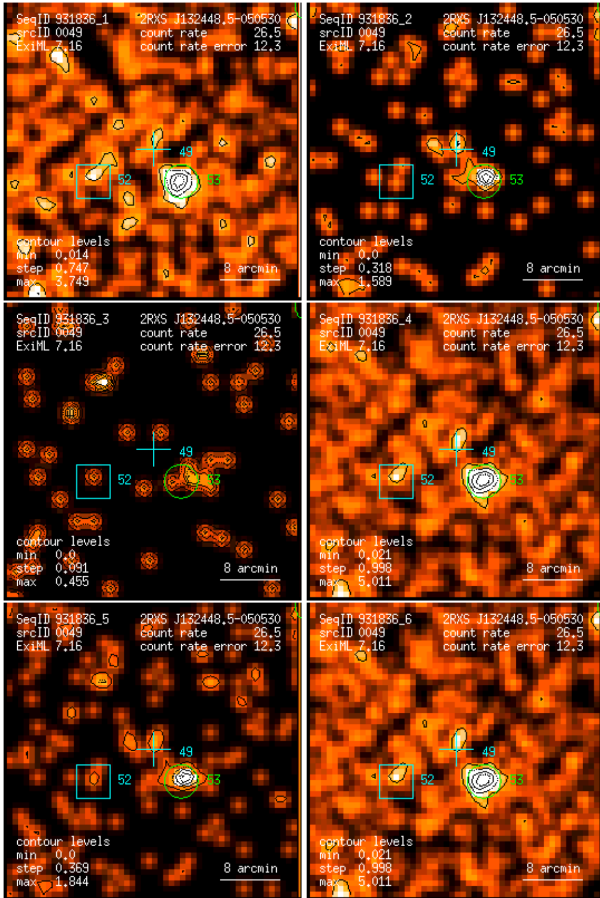
Figure 49: RASS 931836: detection 0049: band rate images, Gaussian filter: (1) PSPC channels 11 – 41, (2) 52 – 90, (3) 91 – 201, (4) 11 – 235, (5) 52 – 201, (6) 11 – 201. Broad band rates in counts/ks. Band rate contour levels in counts/ks/arcmin 2 .
