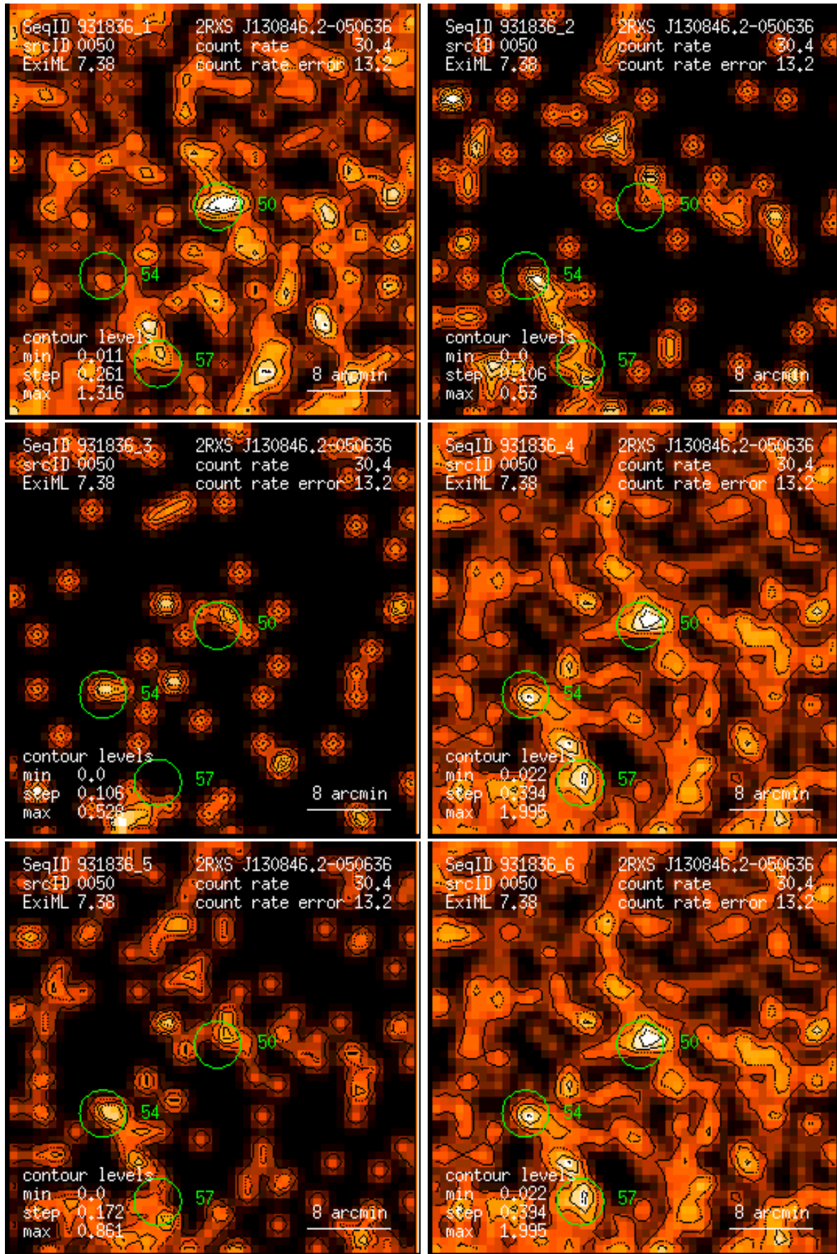
Figure 50: RASS 931836: detection 0050: band rate images, Gaussian filter: (1) PSPC channels 11 – 41, (2) 52 – 90, (3) 91 – 201, (4) 11 – 235, (5) 52 – 201, (6) 11 – 201. Broad band rates in counts/ks. Band rate contour levels in counts/ks/arcmin 2 .
