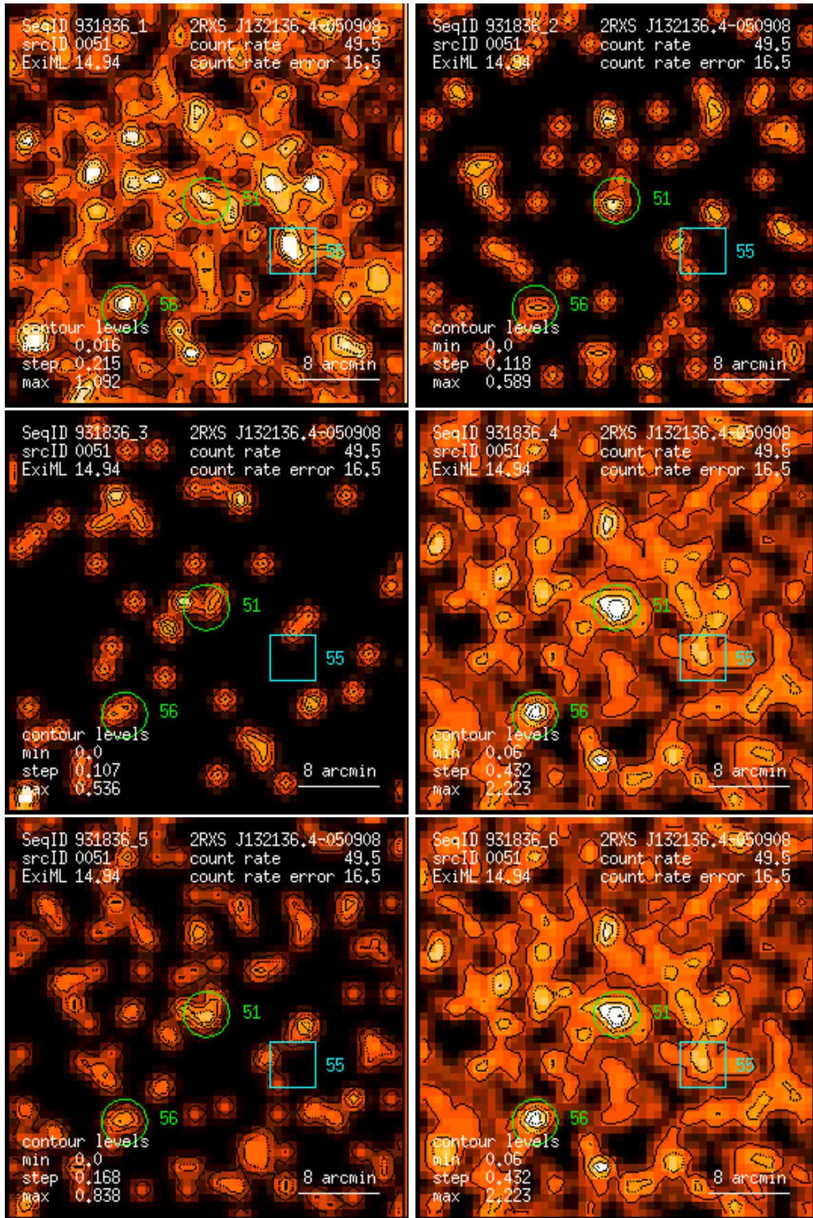
Figure 51: RASS 931836: detection 0051: band rate images, Gaussian filter: (1) PSPC channels 11 – 41, (2) 52 – 90, (3) 91 – 201, (4) 11 – 235, (5) 52 – 201, (6) 11 – 201. Broad band rates in counts/ks. Band rate contour levels in counts/ks/arcmin 2 .
