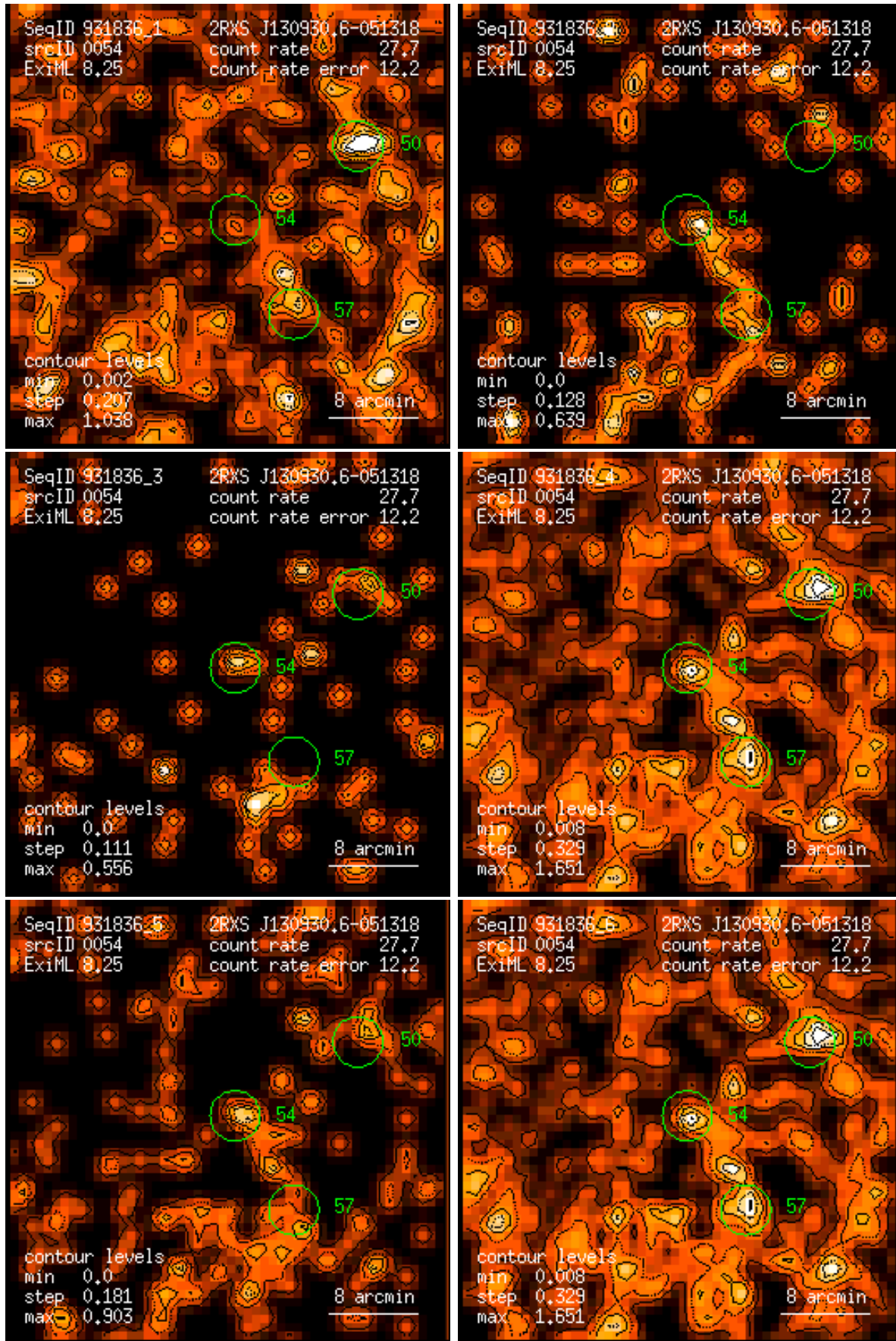
Figure 54: RASS 931836: detection 0054: band rate images, Gaussian filter: (1) PSPC channels 11 – 41, (2) 52 – 90, (3) 91 – 201, (4) 11 – 235, (5) 52 – 201, (6) 11 – 201. Broad band rates in counts/ks. Band rate contour levels in counts/ks/arcmin 2 .
