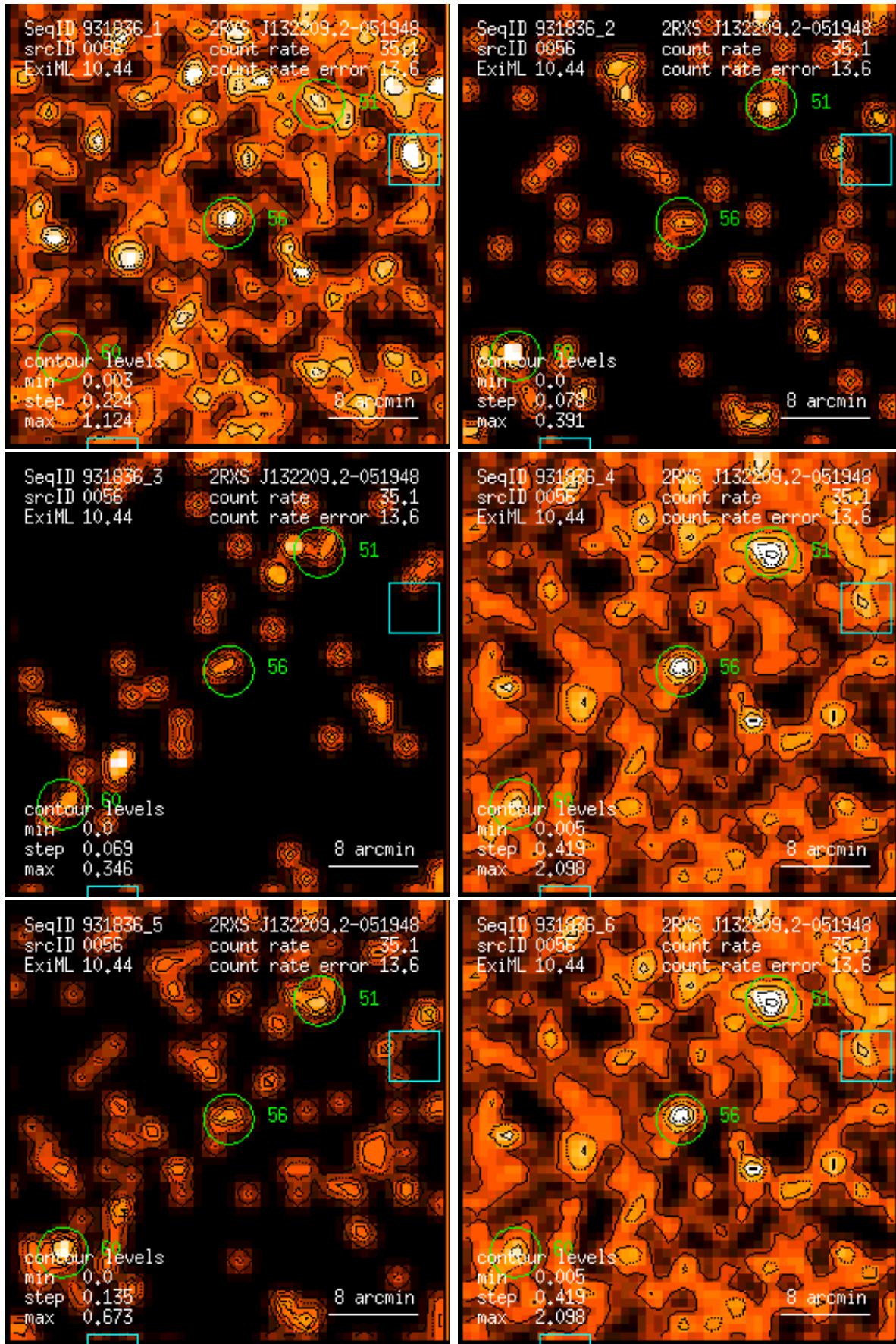
Figure 56: RASS 931836: detection 0056: band rate images, Gaussian filter: (1) PSPC channels 11 – 41, (2) 52 – 90, (3) 91 – 201, (4) 11 – 235, (5) 52 – 201, (6) 11 – 201. Broad band rates in counts/ks. Band rate contour levels in counts/ks/arcmin 2 .
