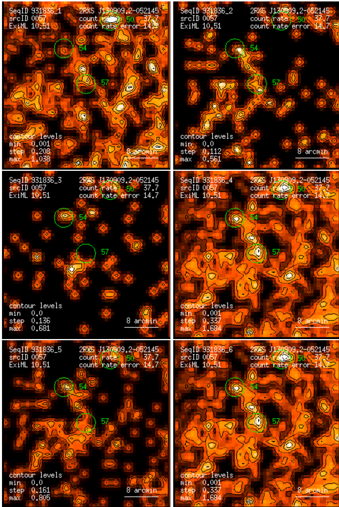
Figure 57: RASS 931836: detection 0057: band rate images, Gaussian filter: (1) PSPC channels 11 – 41, (2) 52 – 90, (3) 91 – 201, (4) 11 – 235, (5) 52 – 201, (6) 11 – 201. Broad band rates in counts/ks. Band rate contour levels in counts/ks/arcmin 2 .
