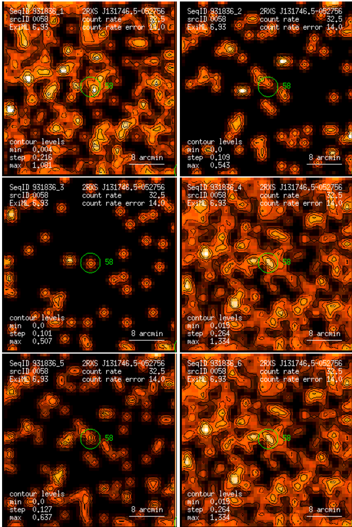
Figure 58: RASS 931836: detection 0058: band rate images, Gaussian filter: (1) PSPC channels 11 – 41, (2) 52 – 90, (3) 91 – 201, (4) 11 – 235, (5) 52 – 201, (6) 11 – 201. Broad band rates in counts/ks. Band rate contour levels in counts/ks/arcmin 2 .
