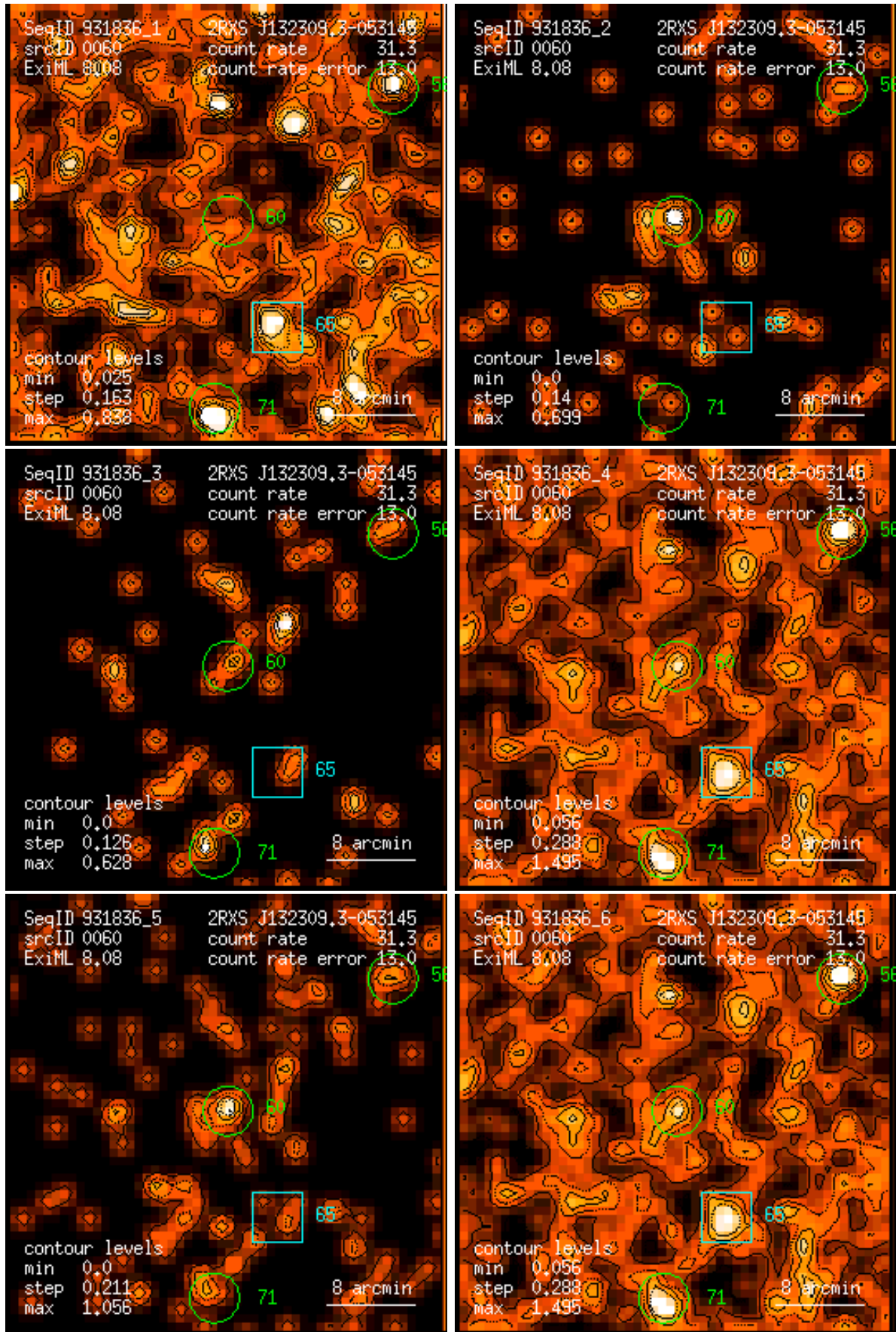
Figure 60: RASS 931836: detection 0060: band rate images, Gaussian filter: (1) PSPC channels 11 – 41, (2) 52 – 90, (3) 91 – 201, (4) 11 – 235, (5) 52 – 201, (6) 11 – 201. Broad band rates in counts/ks. Band rate contour levels in counts/ks/arcmin 2 .
