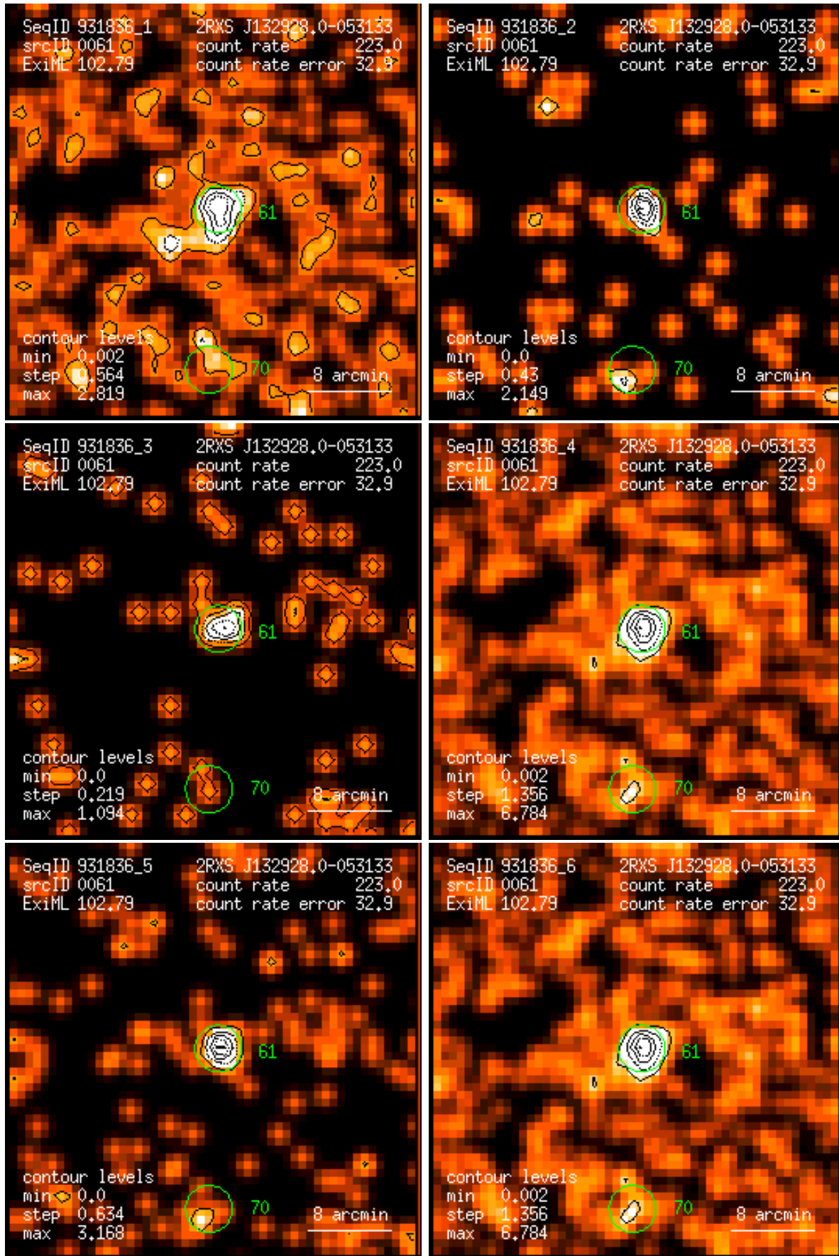
Figure 61: RASS 931836: detection 0061: band rate images, Gaussian filter: (1) PSPC channels 11 – 41, (2) 52 – 90, (3) 91 – 201, (4) 11 – 235, (5) 52 – 201, (6) 11 – 201. Broad band rates in counts/ks. Band rate contour levels in counts/ks/arcmin 2 .
