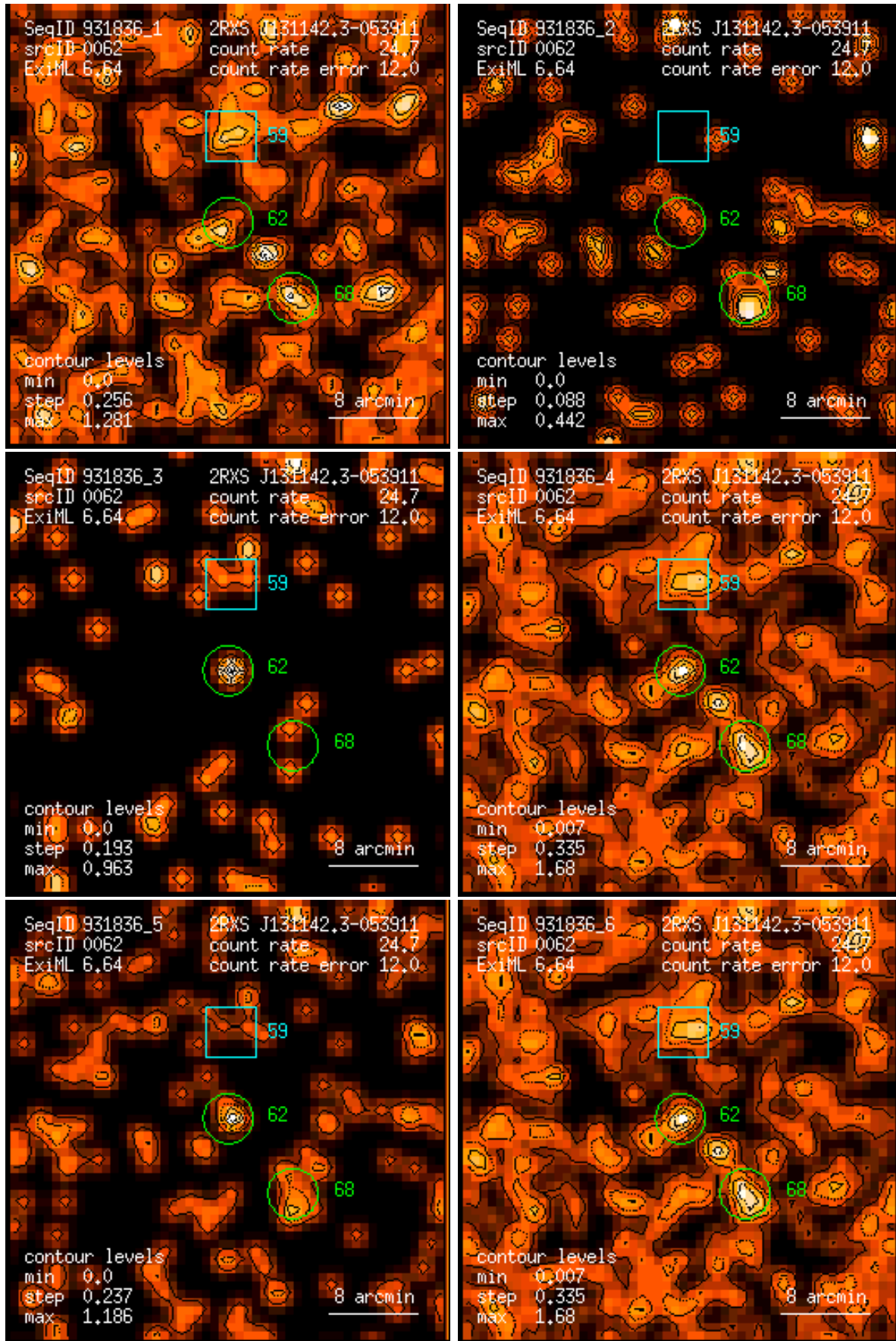
Figure 62: RASS 931836: detection 0062: band rate images, Gaussian filter: (1) PSPC channels 11 – 41, (2) 52 – 90, (3) 91 – 201, (4) 11 – 235, (5) 52 – 201, (6) 11 – 201. Broad band rates in counts/ks. Band rate contour levels in counts/ks/arcmin 2 .
