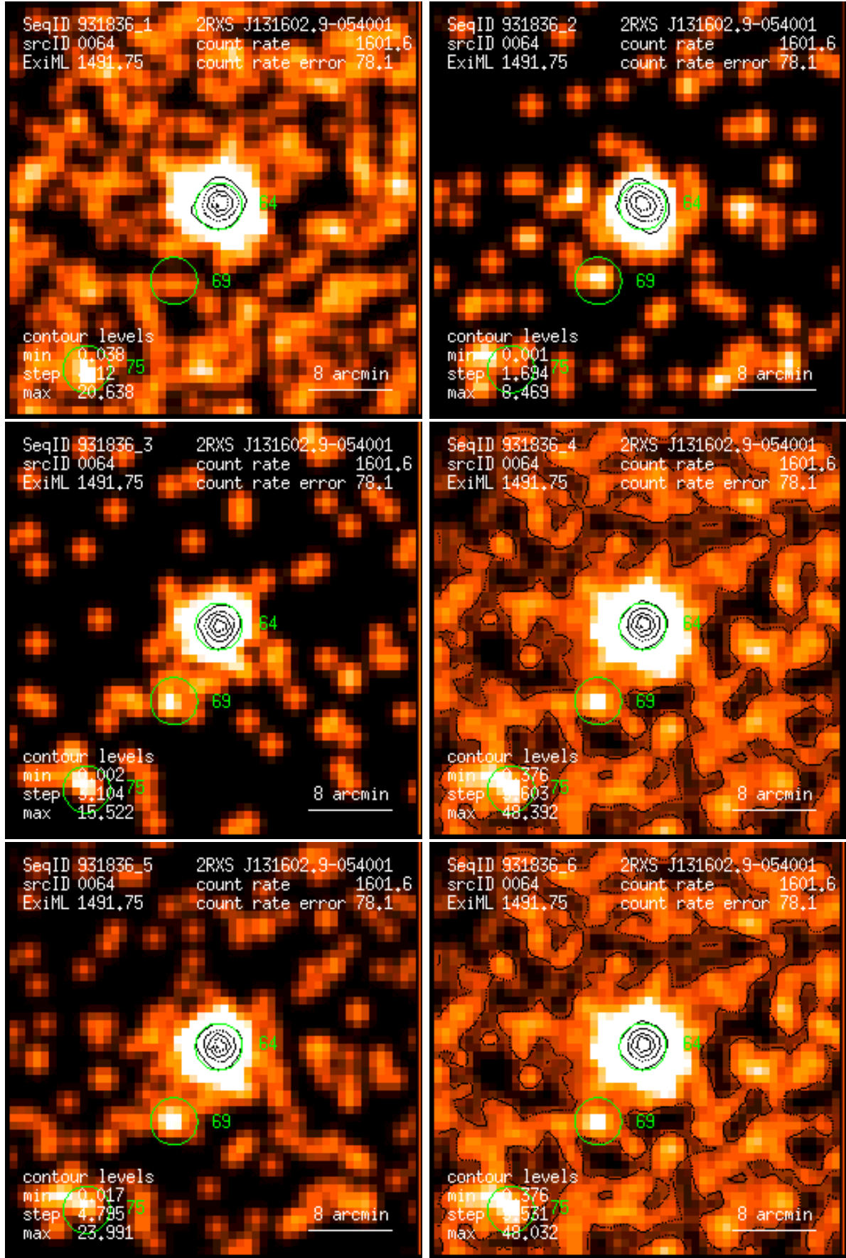
Figure 64: RASS 931836: detection 0064: band rate images, Gaussian filter: (1) PSPC channels 11 – 41, (2) 52 – 90, (3) 91 – 201, (4) 11 – 235, (5) 52 – 201, (6) 11 – 201. Broad band rates in counts/ks. Band rate contour levels in counts/ks/arcmin 2 .
