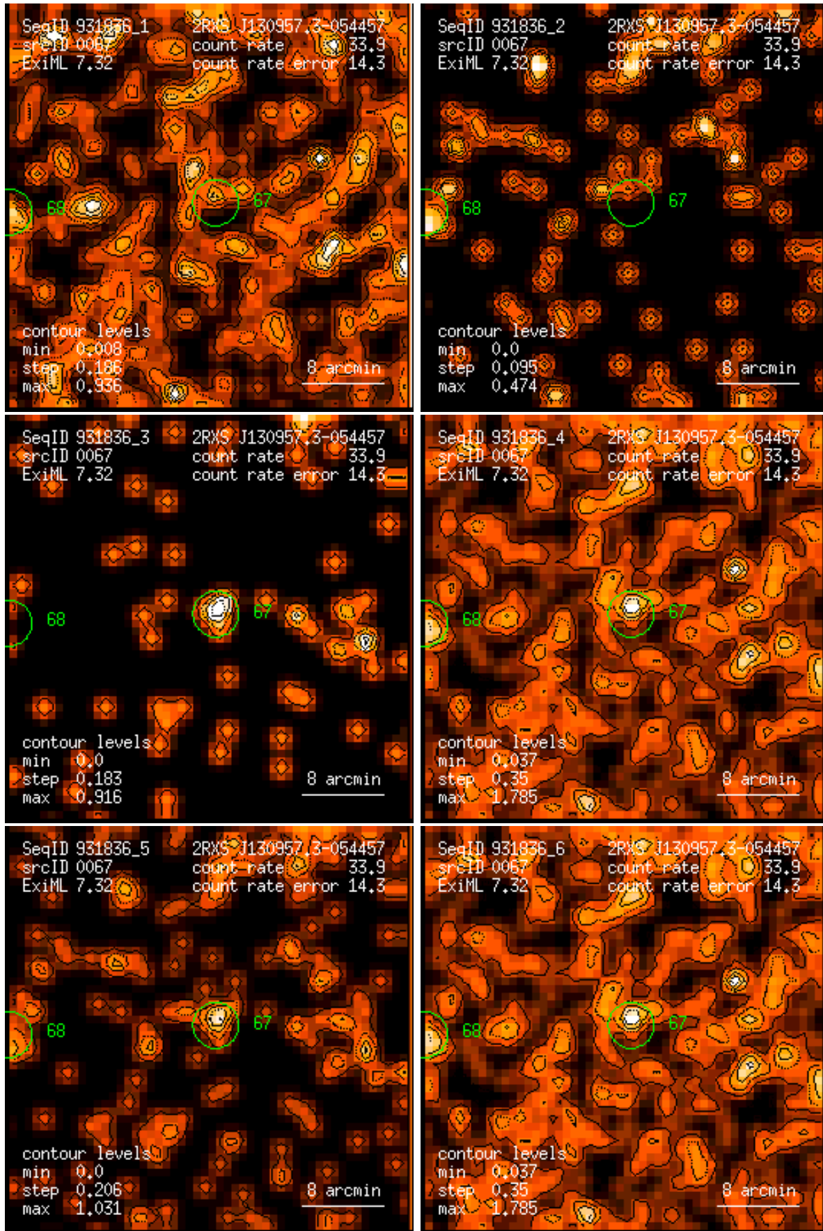
Figure 67: RASS 931836: detection 0067: band rate images, Gaussian filter: (1) PSPC channels 11 – 41, (2) 52 – 90, (3) 91 – 201, (4) 11 – 235, (5) 52 – 201, (6) 11 – 201. Broad band rates in counts/ks. Band rate contour levels in counts/ks/arcmin 2 .
