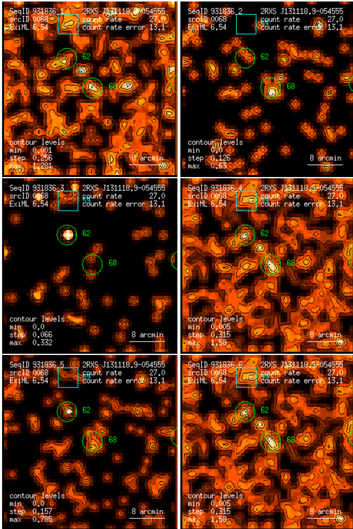
Figure 68: RASS 931836: detection 0068: band rate images, Gaussian filter: (1) PSPC channels 11 – 41, (2) 52 – 90, (3) 91 – 201, (4) 11 – 235, (5) 52 – 201, (6) 11 – 201. Broad band rates in counts/ks. Band rate contour levels in counts/ks/arcmin 2 .
