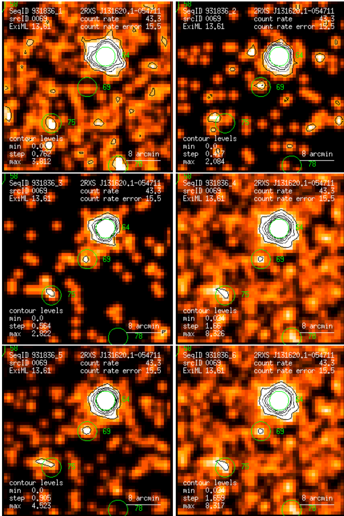
Figure 69: RASS 931836: detection 0069: band rate images, Gaussian filter: (1) PSPC channels 11 – 41, (2) 52 – 90, (3) 91 – 201, (4) 11 – 235, (5) 52 – 201, (6) 11 – 201. Broad band rates in counts/ks. Band rate contour levels in counts/ks/arcmin 2 .
