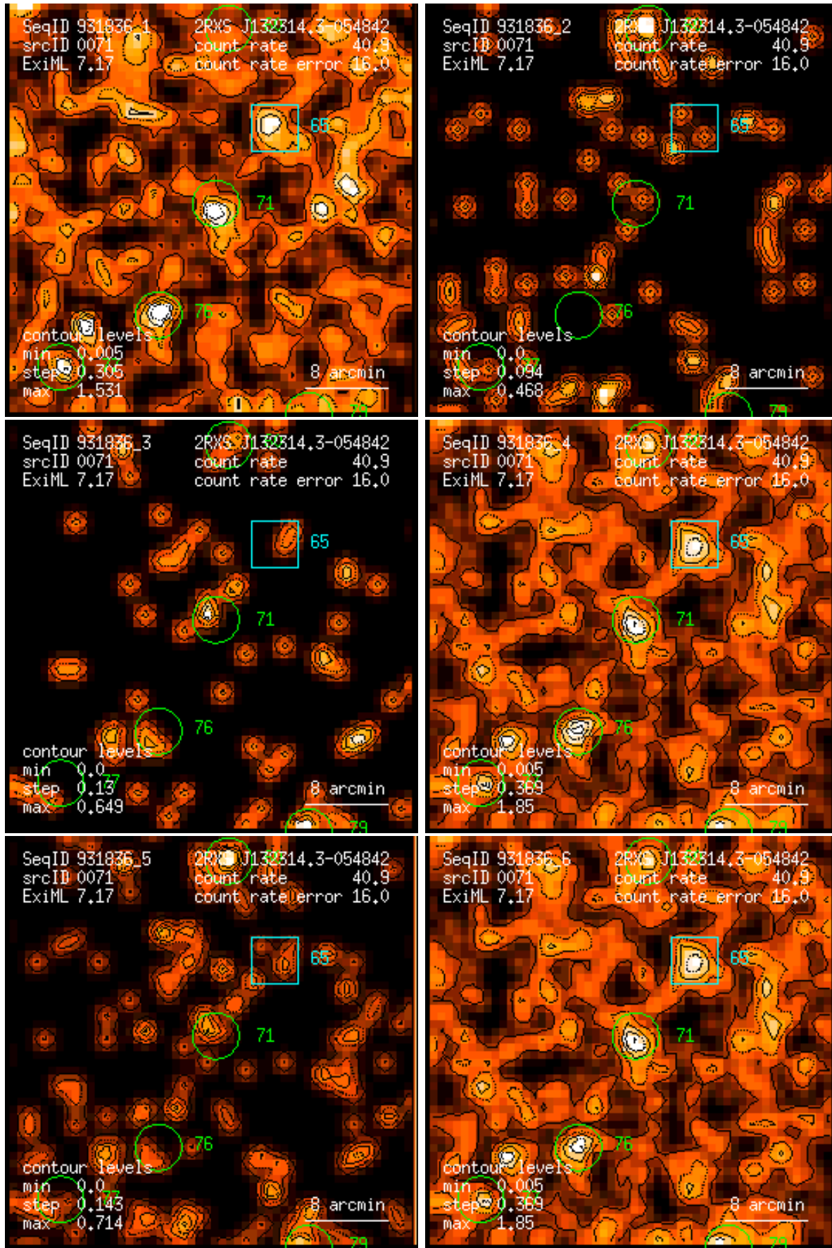
Figure 71: RASS 931836: detection 0071: band rate images, Gaussian filter: (1) PSPC channels 11 – 41, (2) 52 – 90, (3) 91 – 201, (4) 11 – 235, (5) 52 – 201, (6) 11 – 201. Broad band rates in counts/ks. Band rate contour levels in counts/ks/arcmin 2 .
