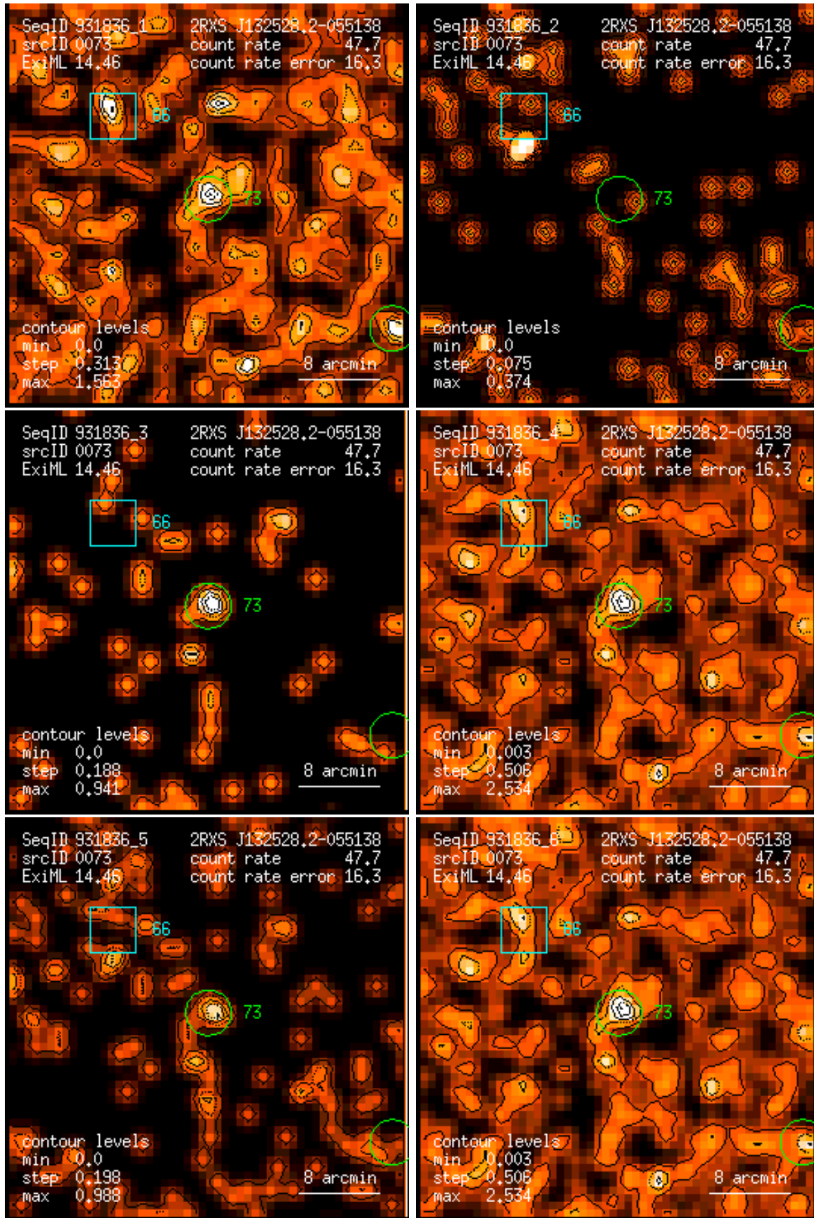
Figure 73: RASS 931836: detection 0073: band rate images, Gaussian filter: (1) PSPC channels 11 – 41, (2) 52 – 90, (3) 91 – 201, (4) 11 – 235, (5) 52 – 201, (6) 11 – 201. Broad band rates in counts/ks. Band rate contour levels in counts/ks/arcmin 2 .
