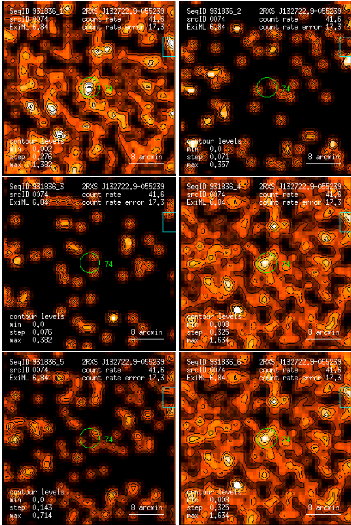
Figure 74: RASS 931836: detection 0074: band rate images, Gaussian filter: (1) PSPC channels 11 – 41, (2) 52 – 90, (3) 91 – 201, (4) 11 – 235, (5) 52 – 201, (6) 11 – 201. Broad band rates in counts/ks. Band rate contour levels in counts/ks/arcmin 2 .
