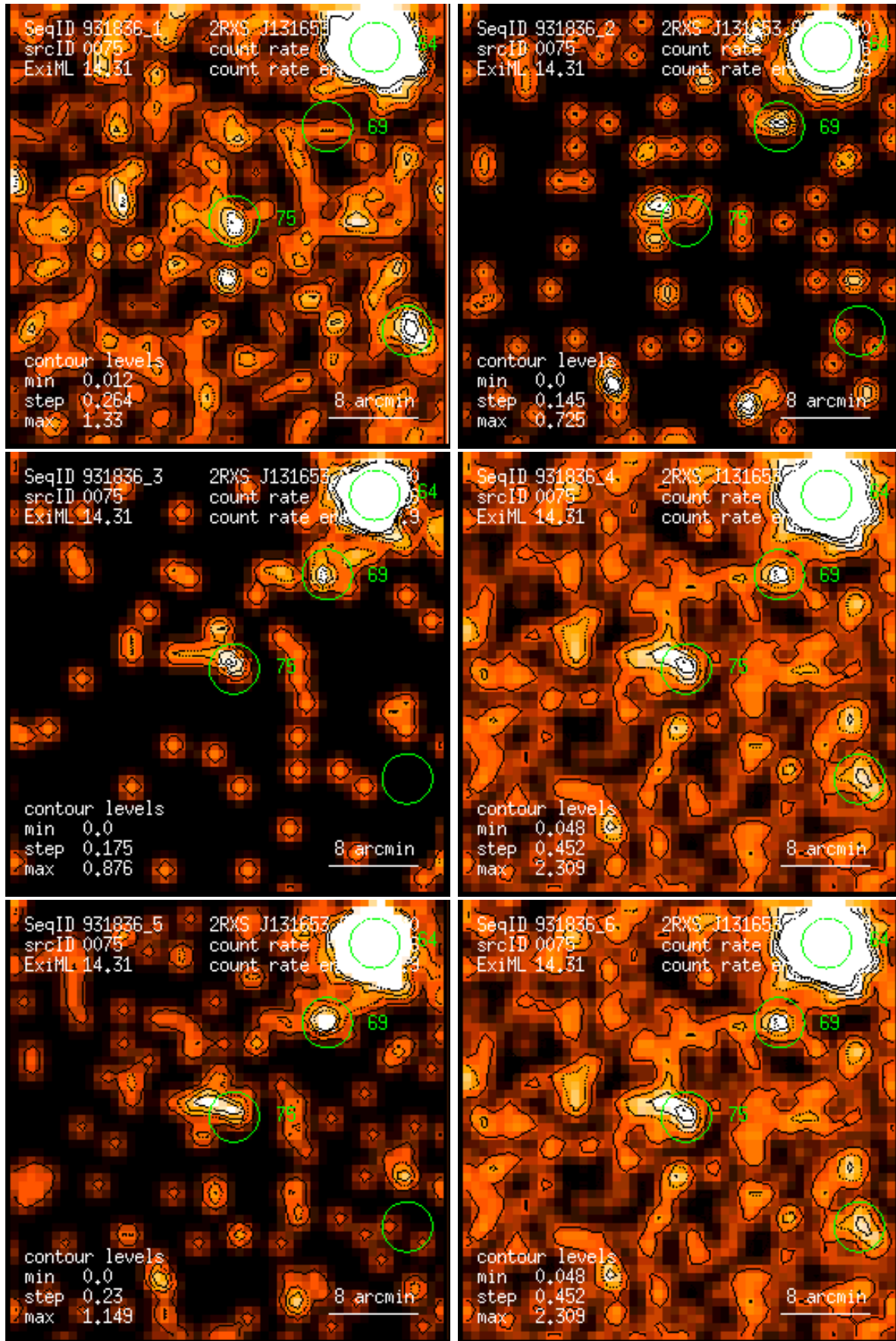
Figure 75: RASS 931836: detection 0075: band rate images, Gaussian filter: (1) PSPC channels 11 – 41, (2) 52 – 90, (3) 91 – 201, (4) 11 – 235, (5) 52 – 201, (6) 11 – 201. Broad band rates in counts/ks. Band rate contour levels in counts/ks/arcmin 2 .
