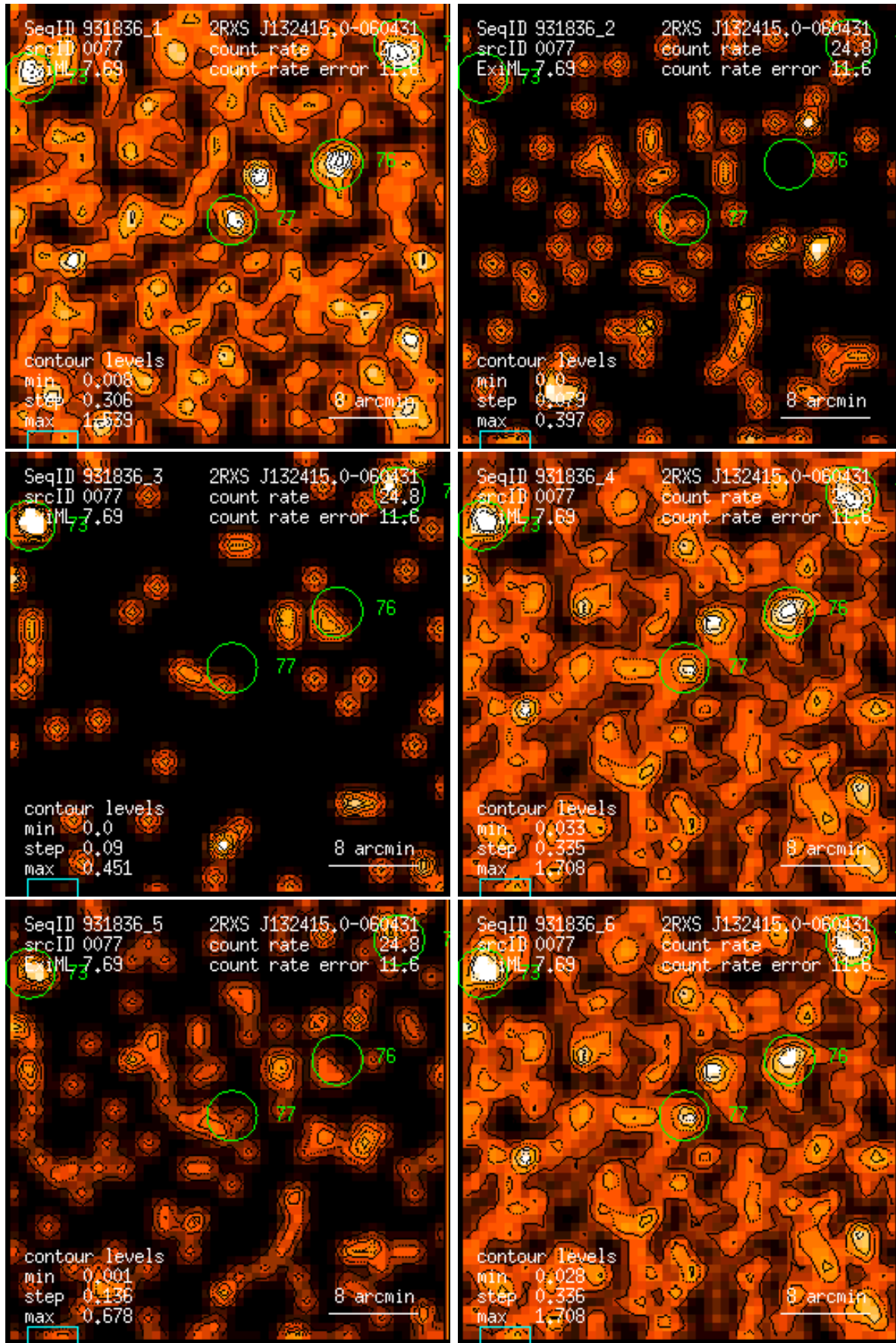
Figure 77: RASS 931836: detection 0077: band rate images, Gaussian filter: (1) PSPC channels 11 – 41, (2) 52 – 90, (3) 91 – 201, (4) 11 – 235, (5) 52 – 201, (6) 11 – 201. Broad band rates in counts/ks. Band rate contour levels in counts/ks/arcmin 2 .
