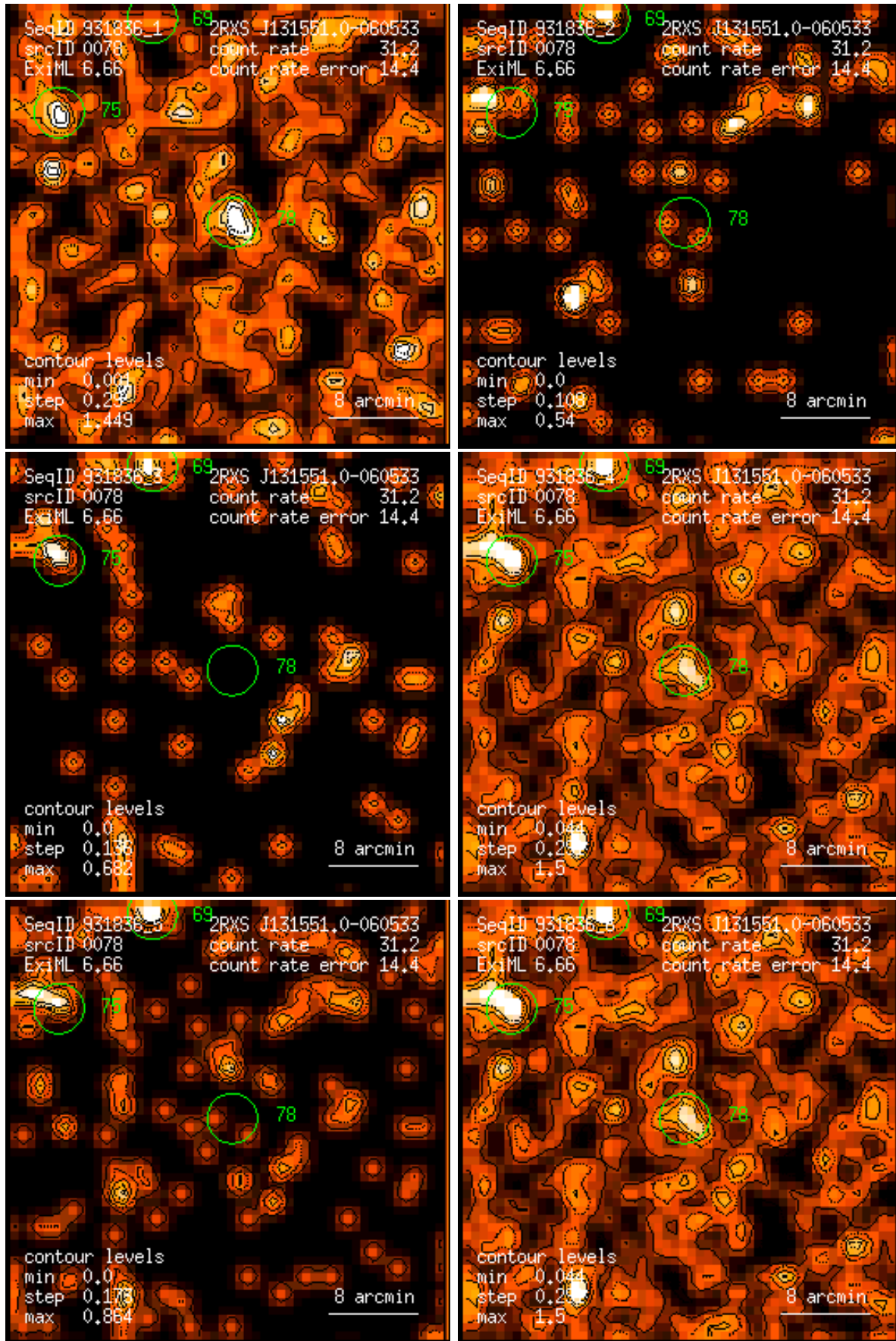
Figure 78: RASS 931836: detection 0078: band rate images, Gaussian filter: (1) PSPC channels 11 – 41, (2) 52 – 90, (3) 91 – 201, (4) 11 – 235, (5) 52 – 201, (6) 11 – 201. Broad band rates in counts/ks. Band rate contour levels in counts/ks/arcmin 2 .
