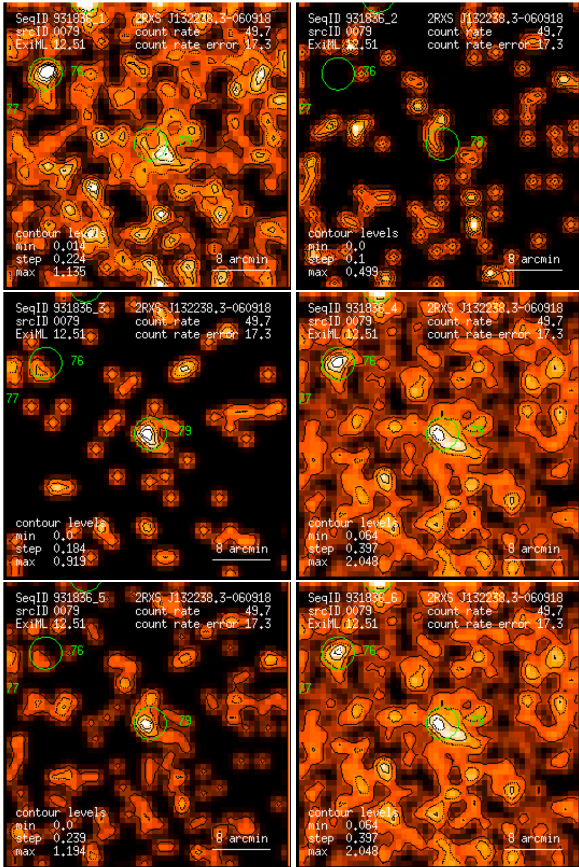
Figure 79: RASS 931836: detection 0079: band rate images, Gaussian filter: (1) PSPC channels 11 – 41, (2) 52 – 90, (3) 91 – 201, (4) 11 – 235, (5) 52 – 201, (6) 11 – 201. Broad band rates in counts/ks. Band rate contour levels in counts/ks/arcmin 2 .
