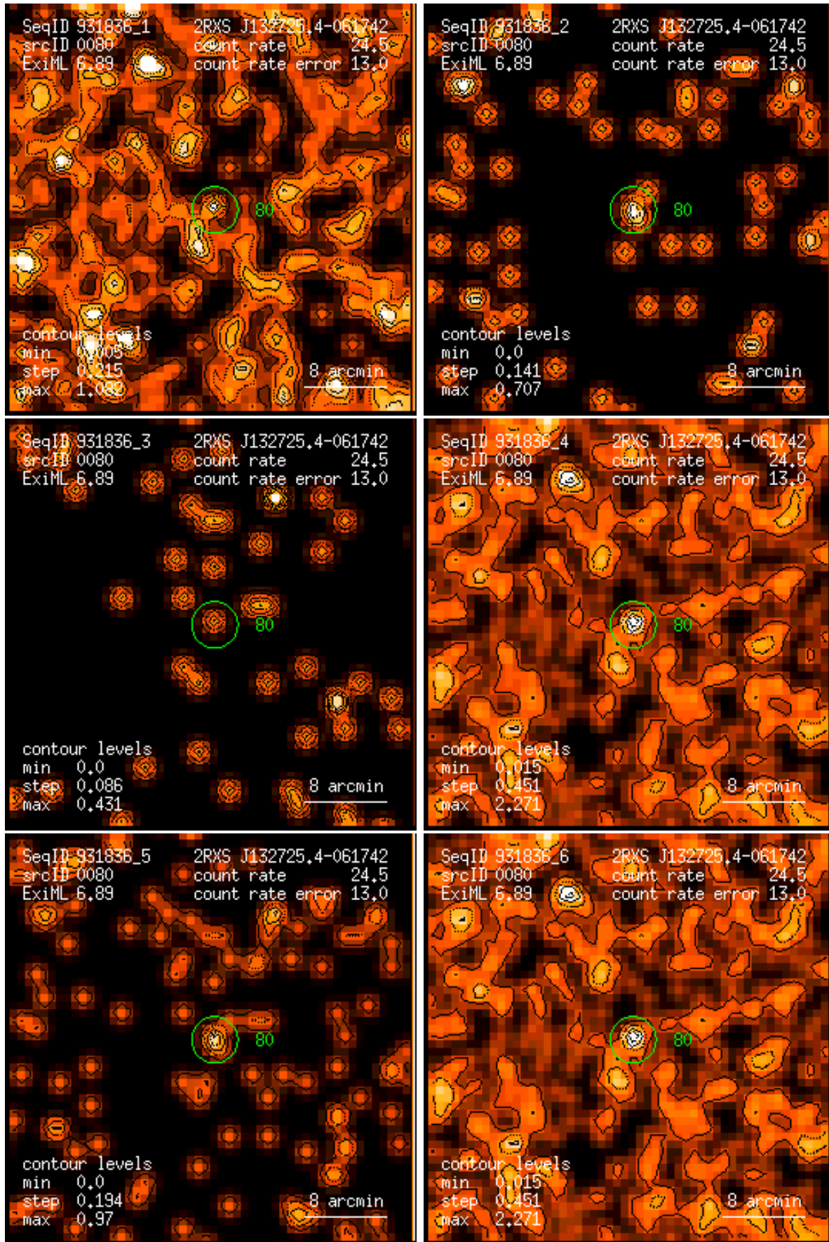
Figure 80: RASS 931836: detection 0080: band rate images, Gaussian filter: (1) PSPC channels 11 – 41, (2) 52 – 90, (3) 91 – 201, (4) 11 – 235, (5) 52 – 201, (6) 11 – 201. Broad band rates in counts/ks. Band rate contour levels in counts/ks/arcmin 2 .
