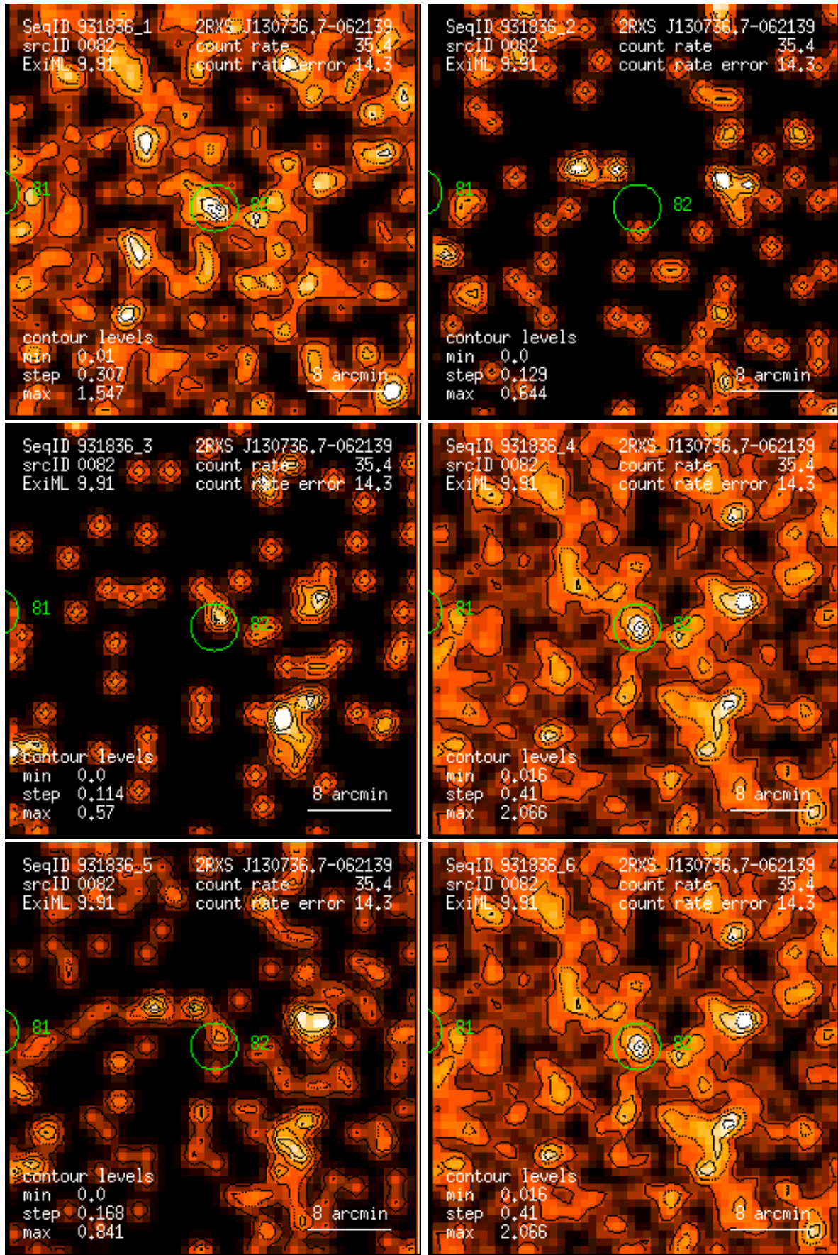
Figure 82: RASS 931836: detection 0082: band rate images, Gaussian filter: (1) PSPC channels 11 – 41, (2) 52 – 90, (3) 91 – 201, (4) 11 – 235, (5) 52 – 201, (6) 11 – 201. Broad band rates in counts/ks. Band rate contour levels in counts/ks/arcmin 2 .
