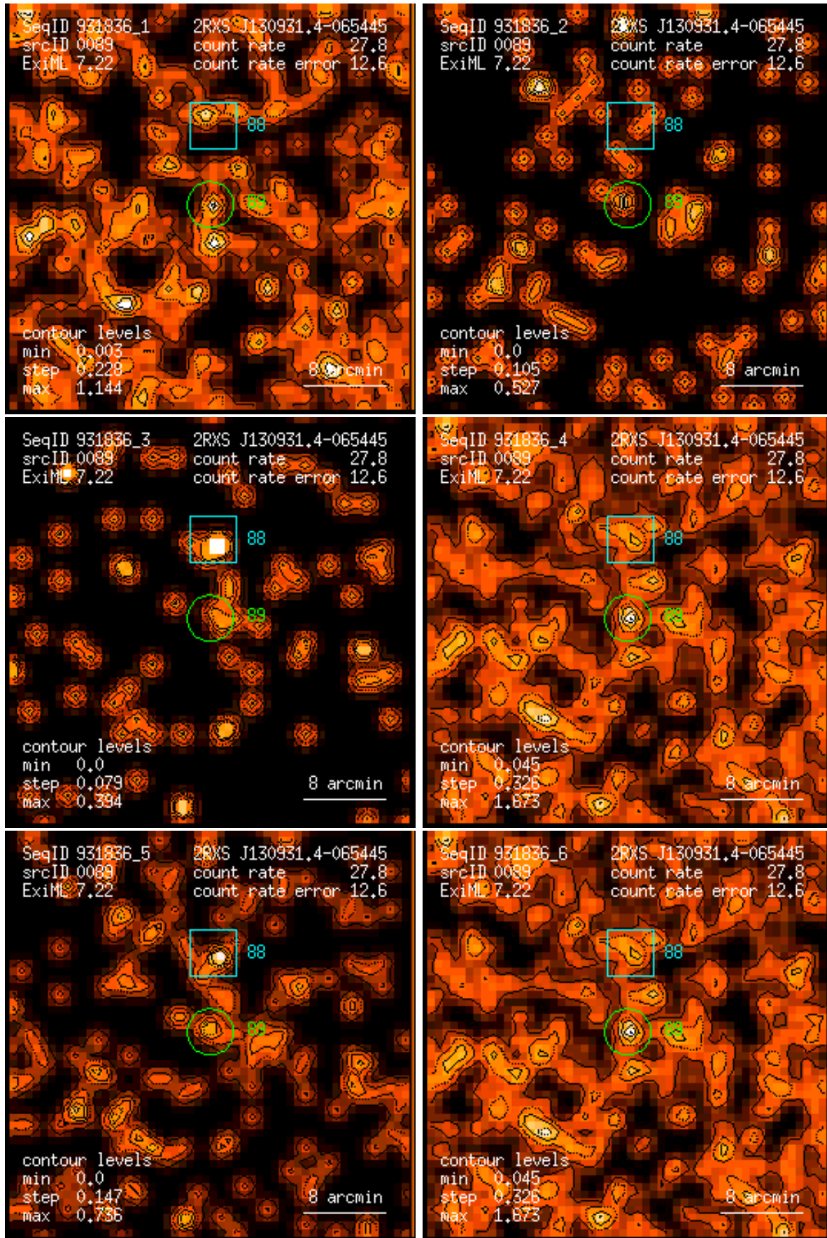
Figure 89: RASS 931836: detection 0089: band rate images, Gaussian filter: (1) PSPC channels 11 – 41, (2) 52 – 90, (3) 91 – 201, (4) 11 – 235, (5) 52 – 201, (6) 11 – 201. Broad band rates in counts/ks. Band rate contour levels in counts/ks/arcmin 2 .
