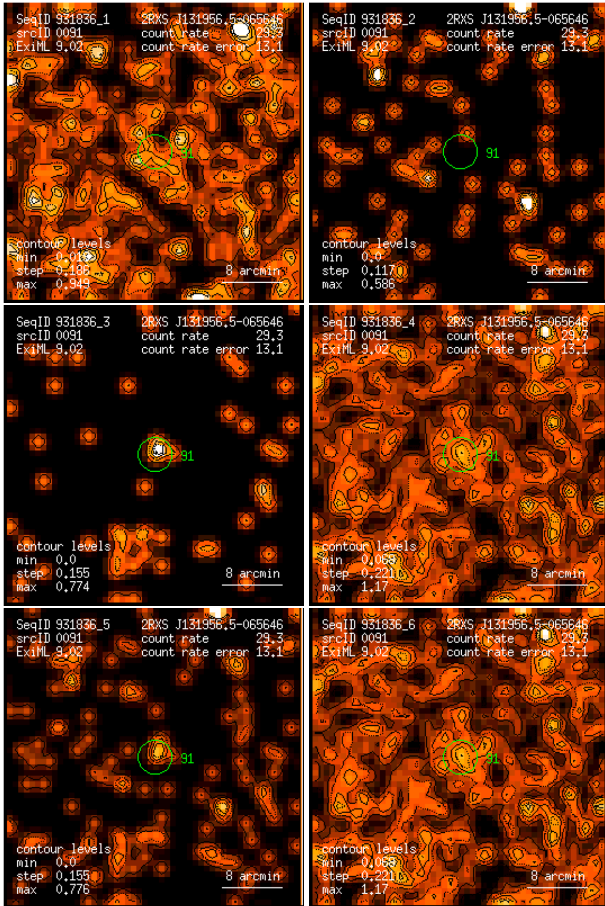
Figure 91: RASS 931836: detection 0091: band rate images, Gaussian filter: (1) PSPC channels 11 – 41, (2) 52 – 90, (3) 91 – 201, (4) 11 – 235, (5) 52 – 201, (6) 11 – 201. Broad band rates in counts/ks. Band rate contour levels in counts/ks/arcmin 2 .
