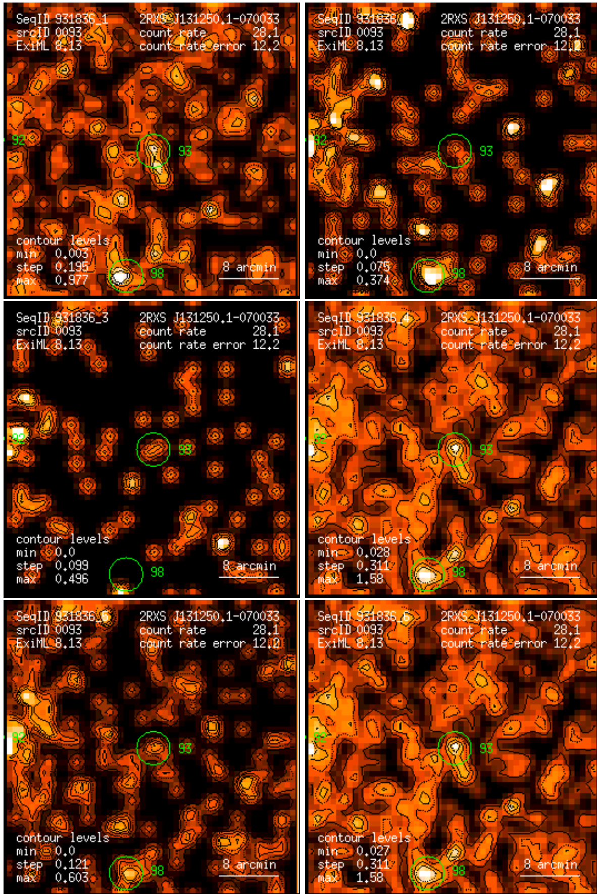
Figure 93: RASS 931836: detection 0093: band rate images, Gaussian filter: (1) PSPC channels 11 – 41, (2) 52 – 90, (3) 91 – 201, (4) 11 – 235, (5) 52 – 201, (6) 11 – 201. Broad band rates in counts/ks. Band rate contour levels in counts/ks/arcmin 2 .
