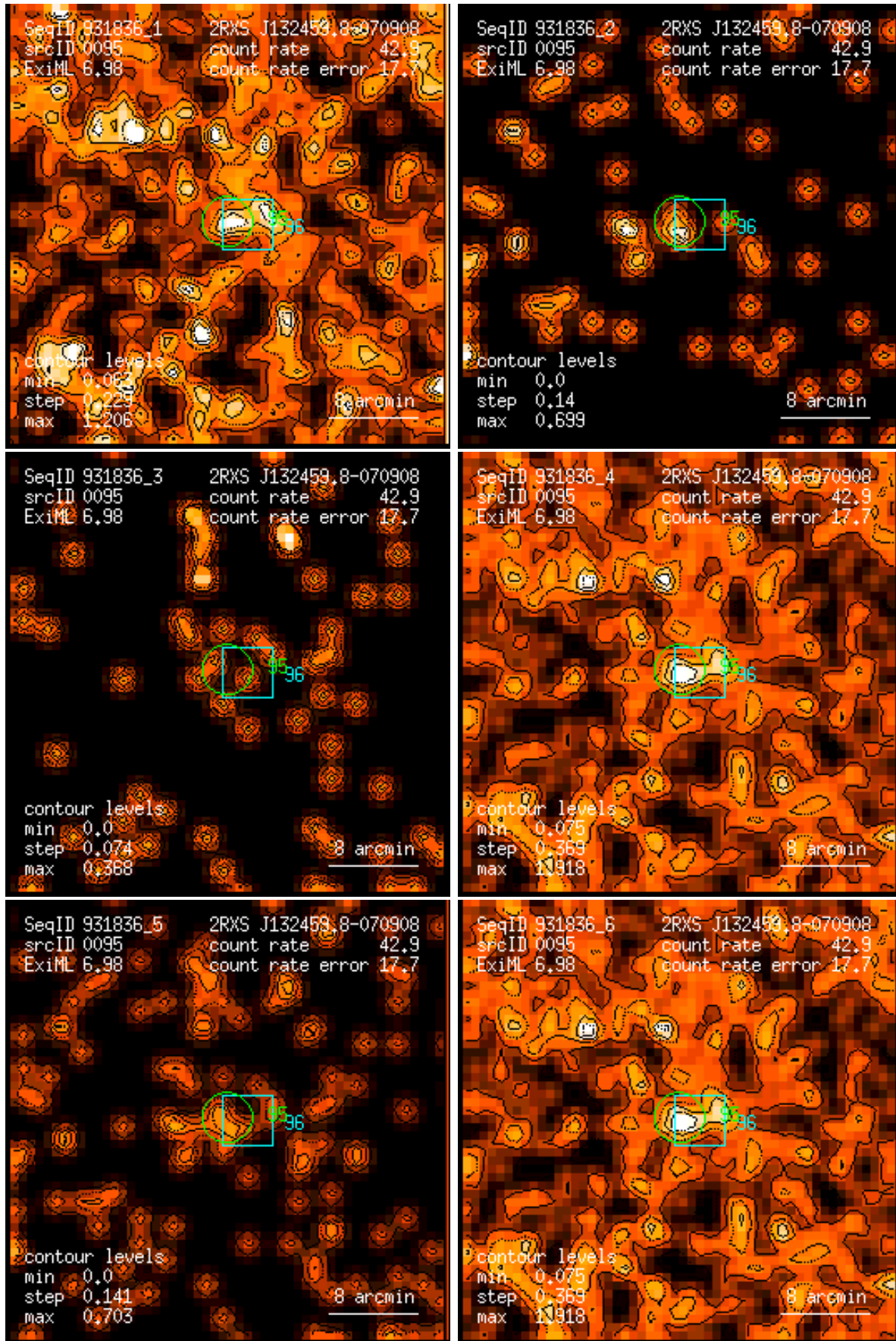
Figure 95: RASS 931836: detection 0095: band rate images, Gaussian filter: (1) PSPC channels 11 – 41, (2) 52 – 90, (3) 91 – 201, (4) 11 – 235, (5) 52 – 201, (6) 11 – 201. Broad band rates in counts/ks. Band rate contour levels in counts/ks/arcmin 2 .
