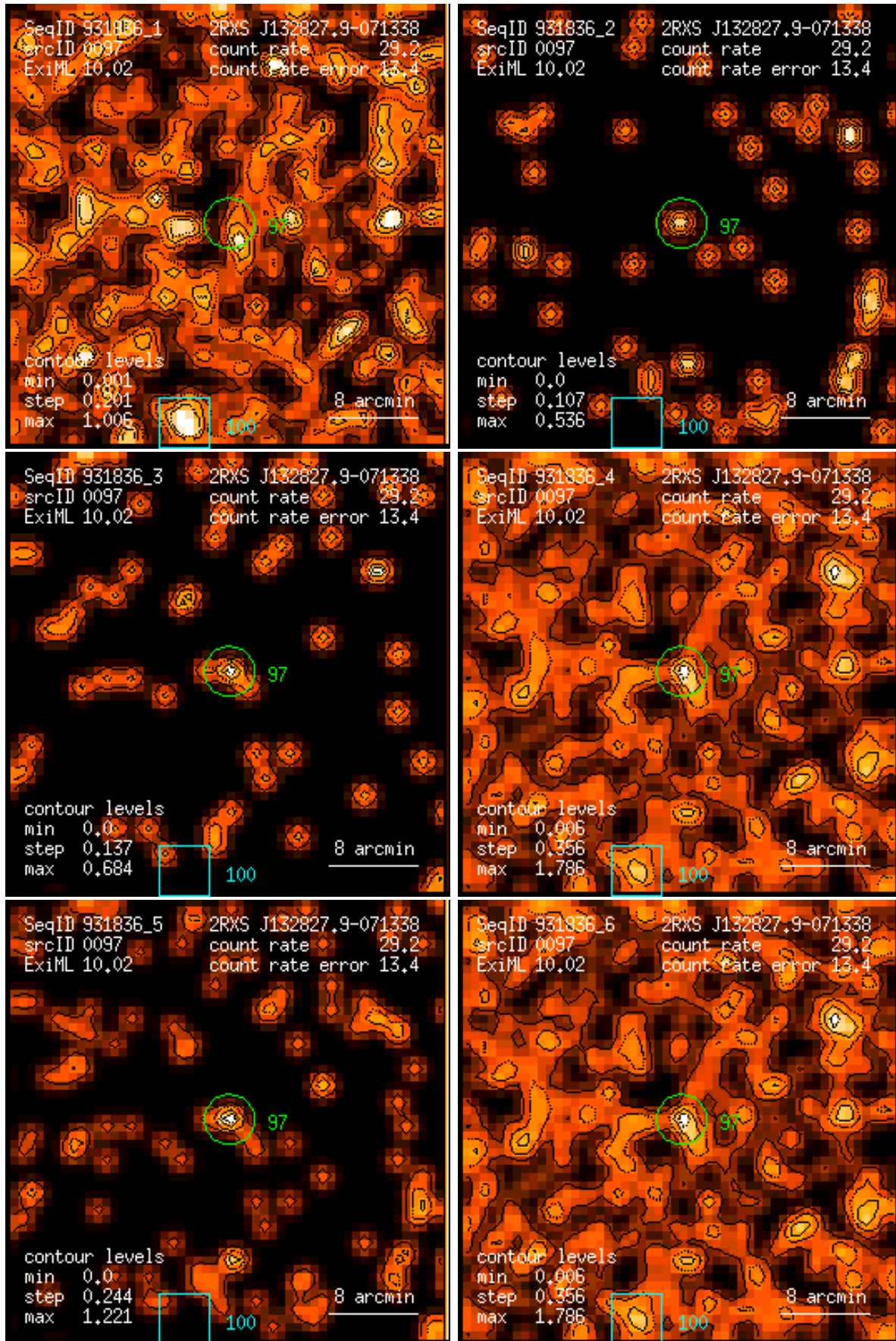
Figure 97: RASS 931836: detection 0097: band rate images, Gaussian filter: (1) PSPC channels 11 – 41, (2) 52 – 90, (3) 91 – 201, (4) 11 – 235, (5) 52 – 201, (6) 11 – 201. Broad band rates in counts/ks. Band rate contour levels in counts/ks/arcmin 2 .
