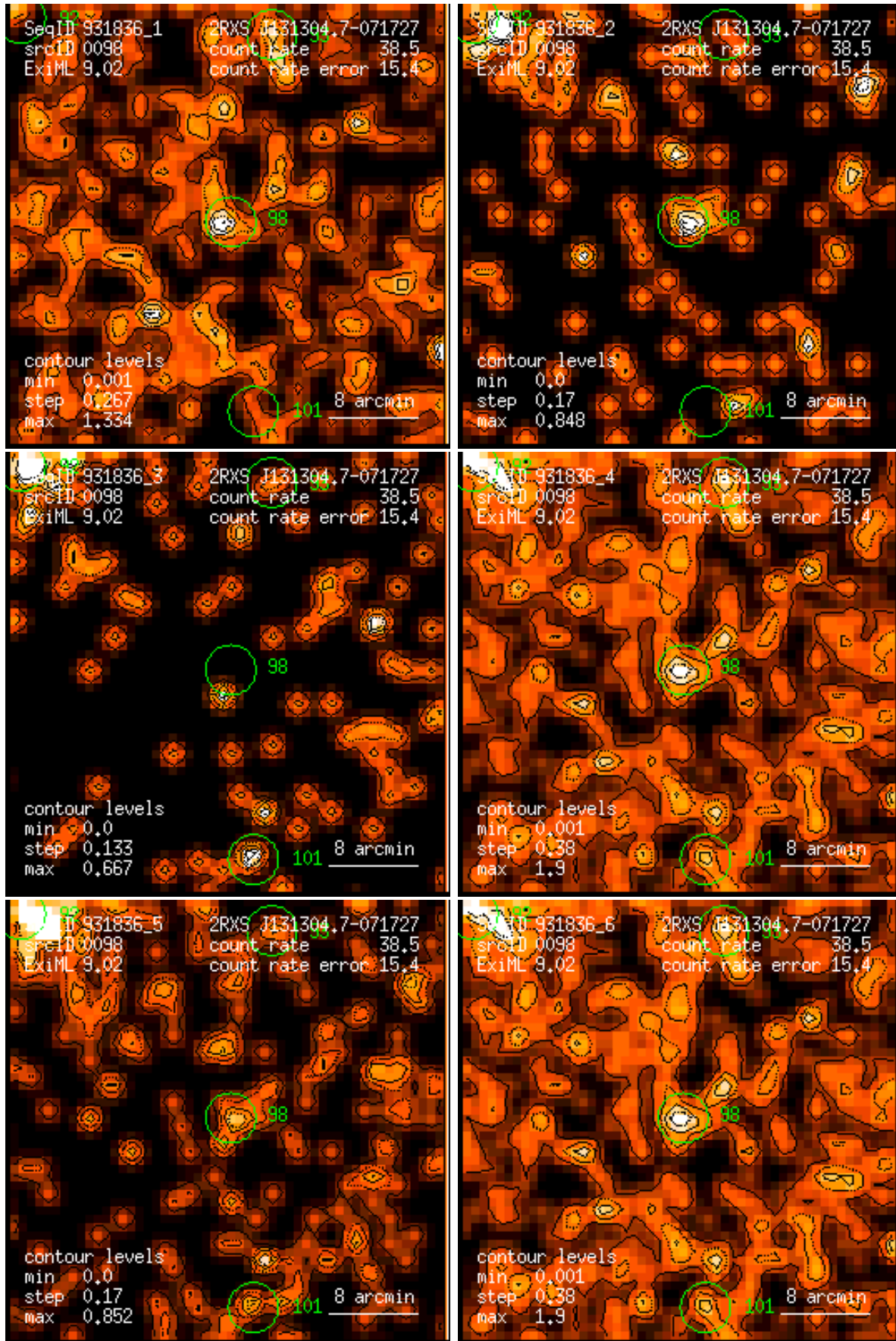
Figure 98: RASS 931836: detection 0098: band rate images, Gaussian filter: (1) PSPC channels 11 – 41, (2) 52 – 90, (3) 91 – 201, (4) 11 – 235, (5) 52 – 201, (6) 11 – 201. Broad band rates in counts/ks. Band rate contour levels in counts/ks/arcmin 2 .
