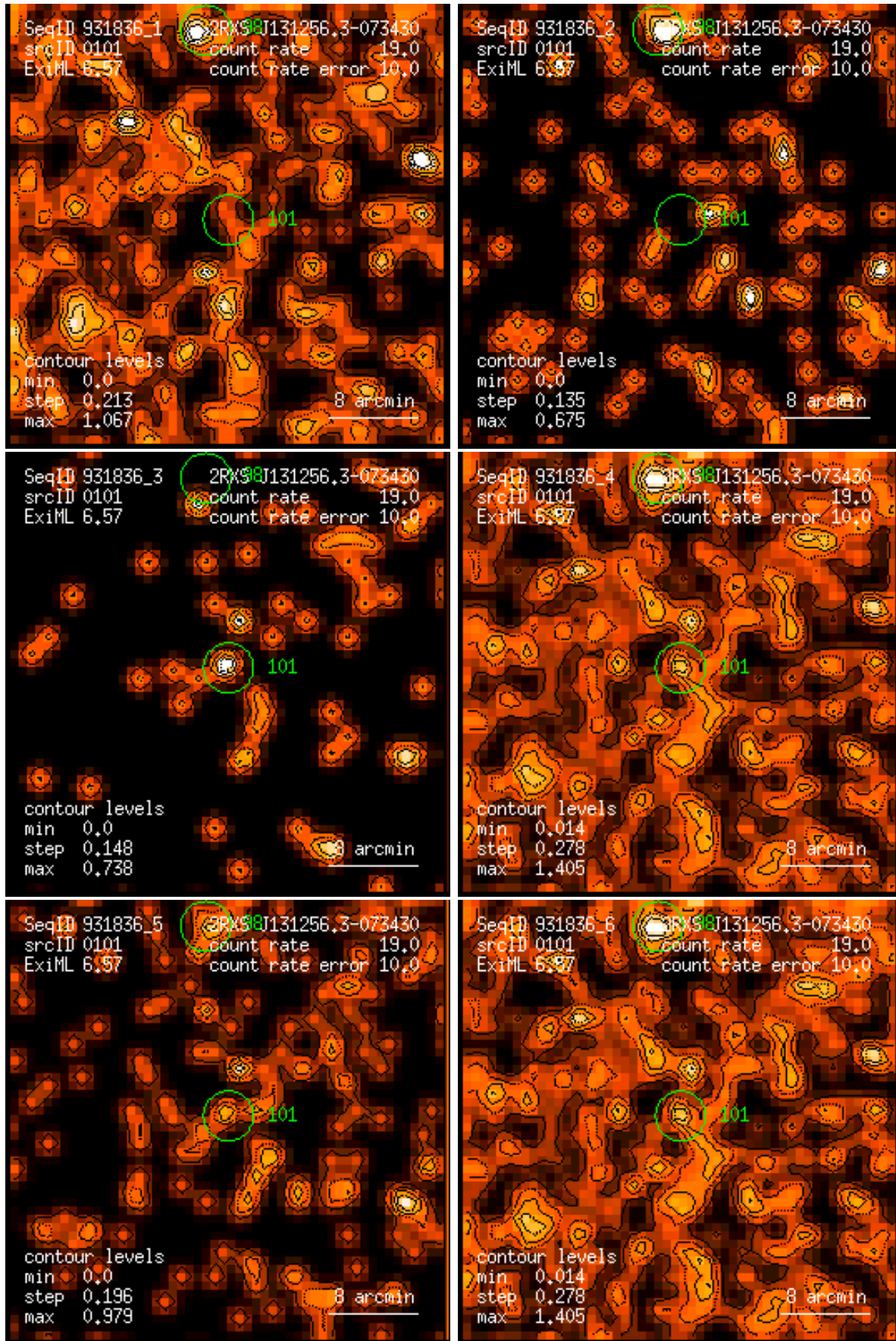
Figure 101: RASS 931836: detection 0101: band rate images, Gaussian filter: (1) PSPC channels 11 – 41, (2) 52 – 90, (3) 91 – 201, (4) 11 – 235, (5) 52 – 201, (6) 11 – 201. Broad band rates in counts/ks. Band rate contour levels in counts/ks/arcmin 2 .
