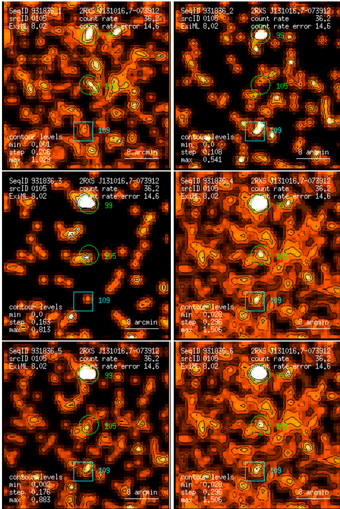
Figure 105: RASS 931836: detection 0105: band rate images, Gaussian filter: (1) PSPC channels 11 – 41, (2) 52 – 90, (3) 91 – 201, (4) 11 – 235, (5) 52 – 201, (6) 11 – 201. Broad band rates in counts/ks. Band rate contour levels in counts/ks/arcmin 2 .
