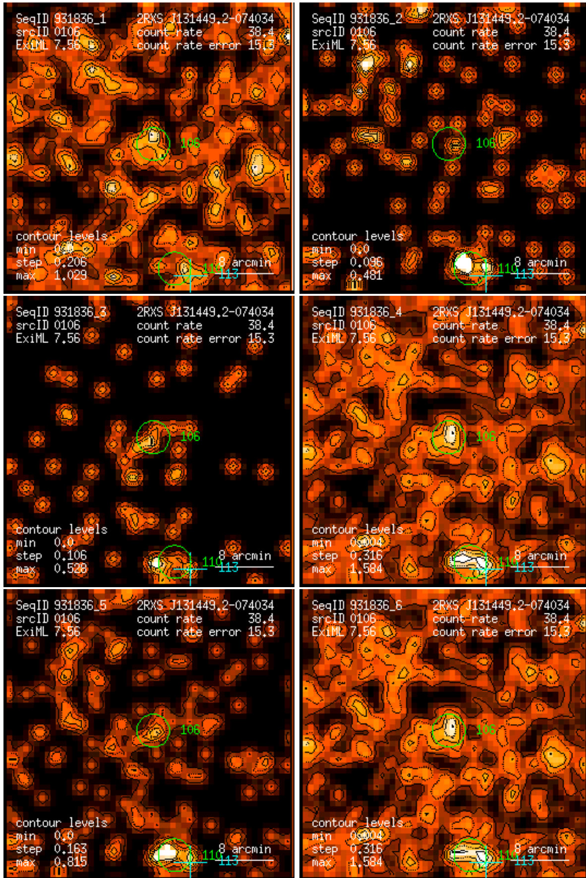
Figure 106: RASS 931836: detection 0106: band rate images, Gaussian filter: (1) PSPC channels 11 – 41, (2) 52 – 90, (3) 91 – 201, (4) 11 – 235, (5) 52 – 201, (6) 11 – 201. Broad band rates in counts/ks. Band rate contour levels in counts/ks/arcmin 2 .
