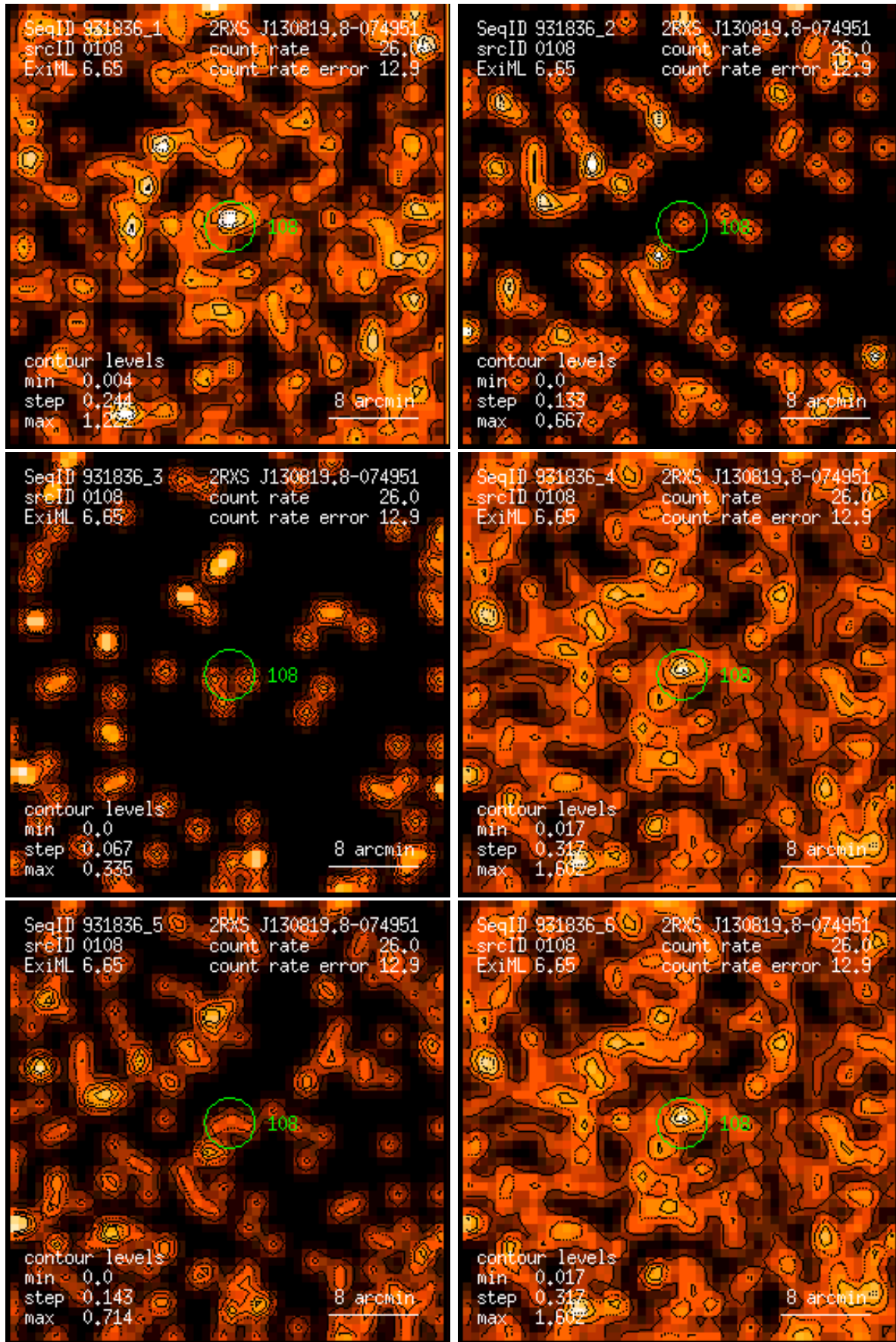
Figure 108: RASS 931836: detection 0108: band rate images, Gaussian filter: (1) PSPC channels 11 – 41, (2) 52 – 90, (3) 91 – 201, (4) 11 – 235, (5) 52 – 201, (6) 11 – 201. Broad band rates in counts/ks. Band rate contour levels in counts/ks/arcmin 2 .
