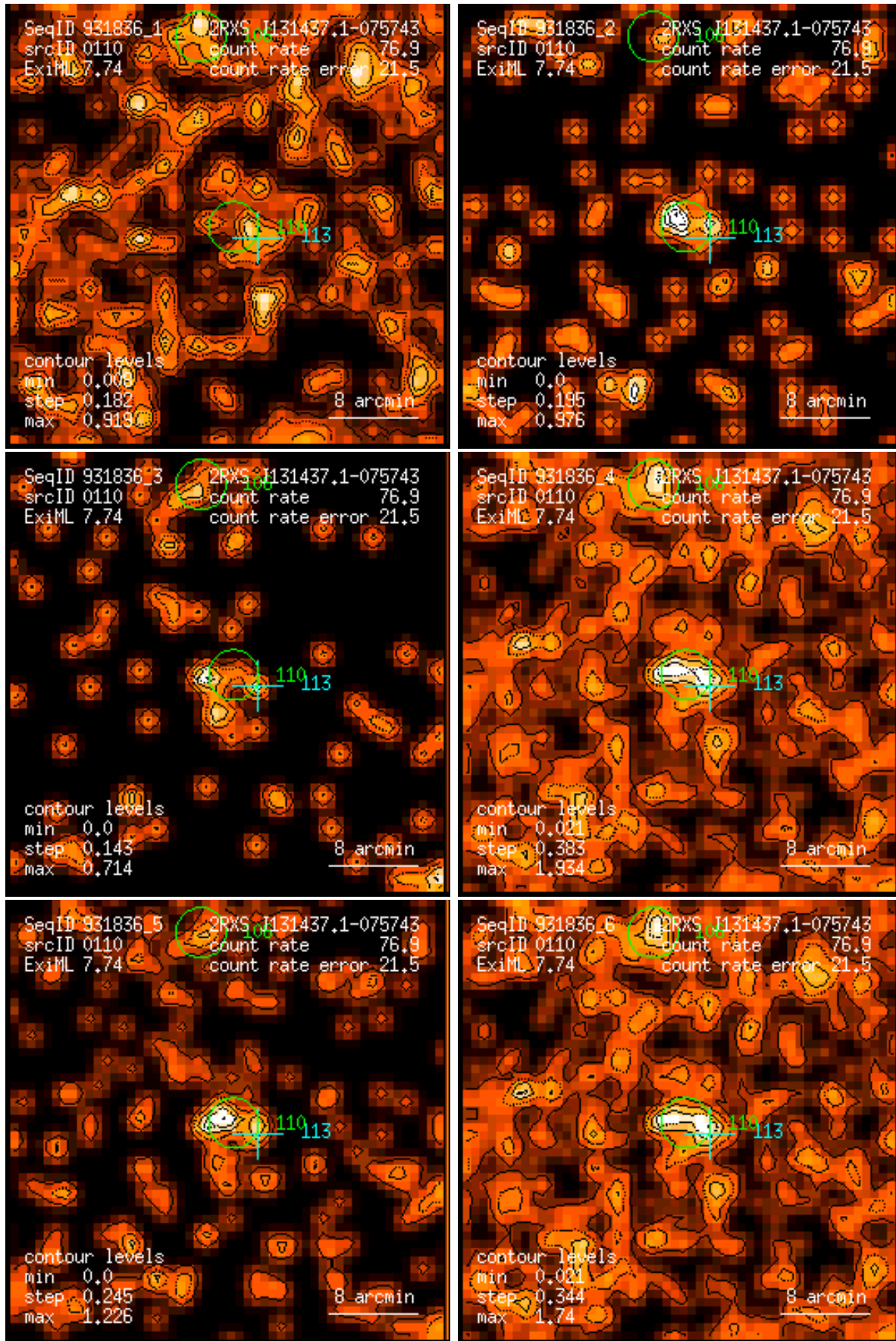
Figure 110: RASS 931836: detection 0110: band rate images, Gaussian filter: (1) PSPC channels 11 – 41, (2) 52 – 90, (3) 91 – 201, (4) 11 – 235, (5) 52 – 201, (6) 11 – 201. Broad band rates in counts/ks. Band rate contour levels in counts/ks/arcmin 2 .
