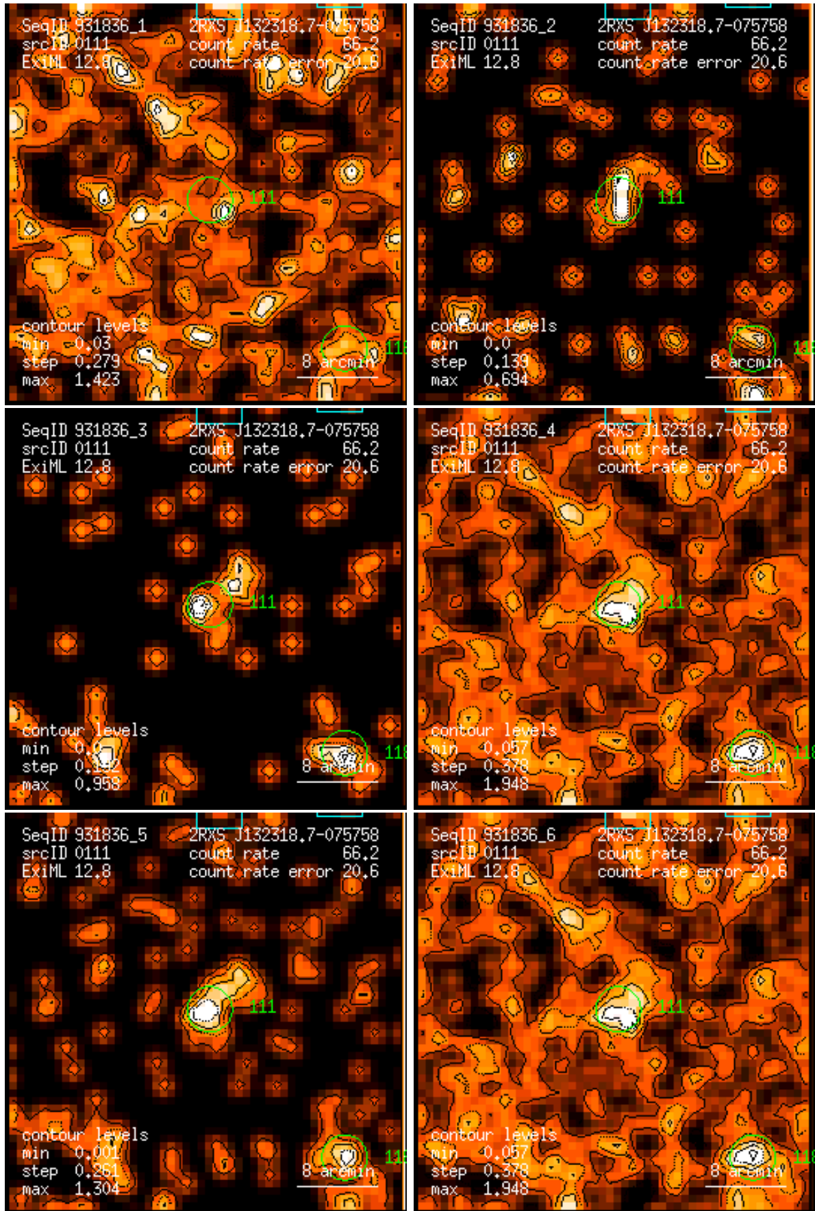
Figure 111: RASS 931836: detection 0111: band rate images, Gaussian filter: (1) PSPC channels 11 – 41, (2) 52 – 90, (3) 91 – 201, (4) 11 – 235, (5) 52 – 201, (6) 11 – 201. Broad band rates in counts/ks. Band rate contour levels in counts/ks/arcmin 2 .
